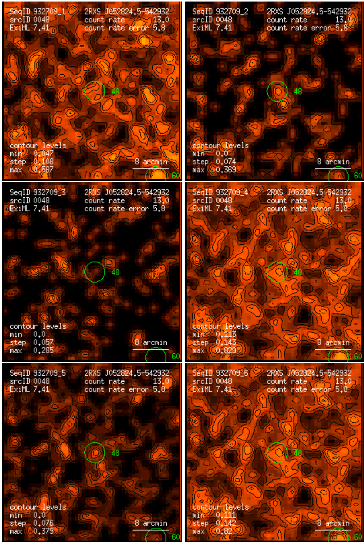
Figure 48: RASS 932709: detection 0048: band rate images, Gaussian filter: (1) PSPC channels 11 – 41, (2) 52 – 90, (3) 91 – 201, (4) 11 – 235, (5) 52 – 201, (6) 11 – 201. Broad band rates in counts/ks. Band rate contour levels in counts/ks/arcmin 2 .
