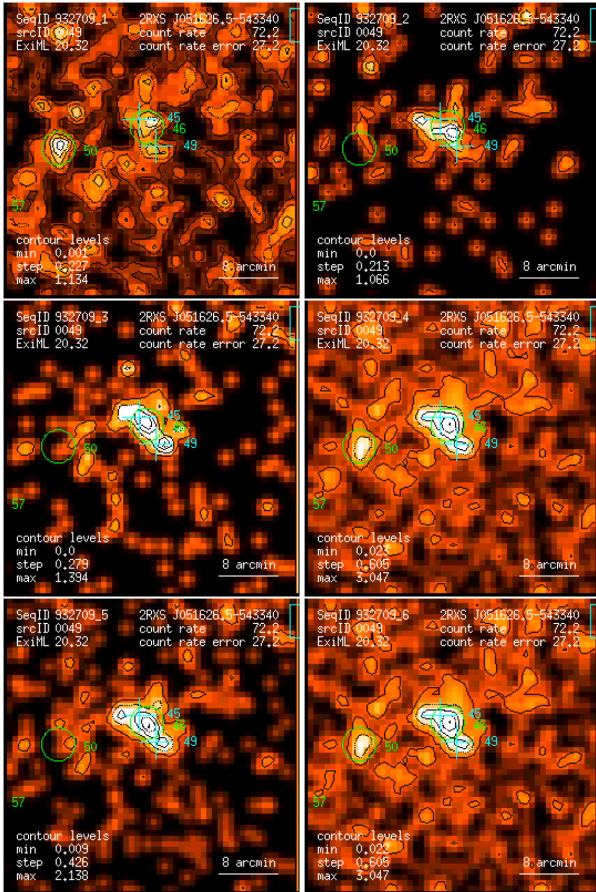
Figure 49: RASS 932709: detection 0049: band rate images, Gaussian filter: (1) PSPC channels 11 – 41, (2) 52 – 90, (3) 91 – 201, (4) 11 – 235, (5) 52 – 201, (6) 11 – 201. Broad band rates in counts/ks. Band rate contour levels in counts/ks/arcmin 2 .
