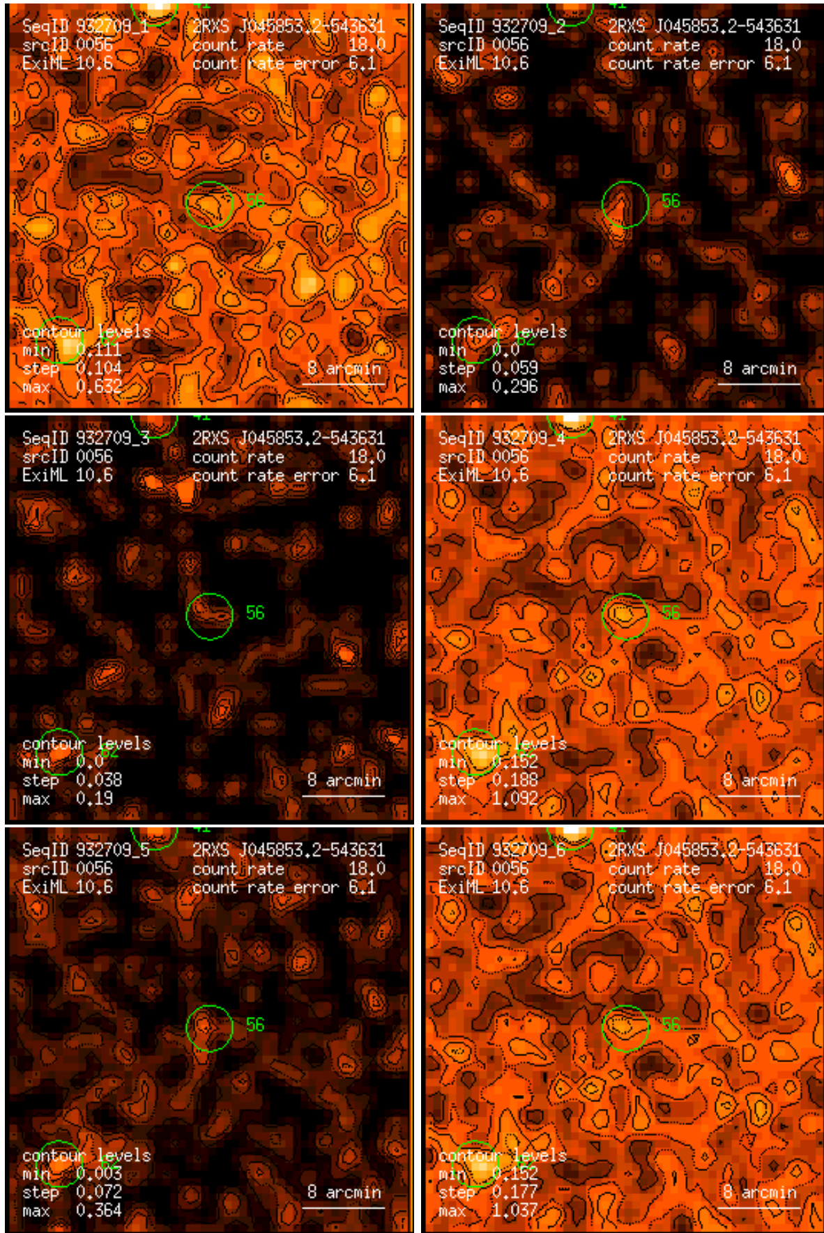
Figure 56: RASS 932709: detection 0056: band rate images, Gaussian filter: (1) PSPC channels 11 – 41, (2) 52 – 90, (3) 91 – 201, (4) 11 – 235, (5) 52 – 201, (6) 11 – 201. Broad band rates in counts/ks. Band rate contour levels in counts/ks/arcmin 2 .
