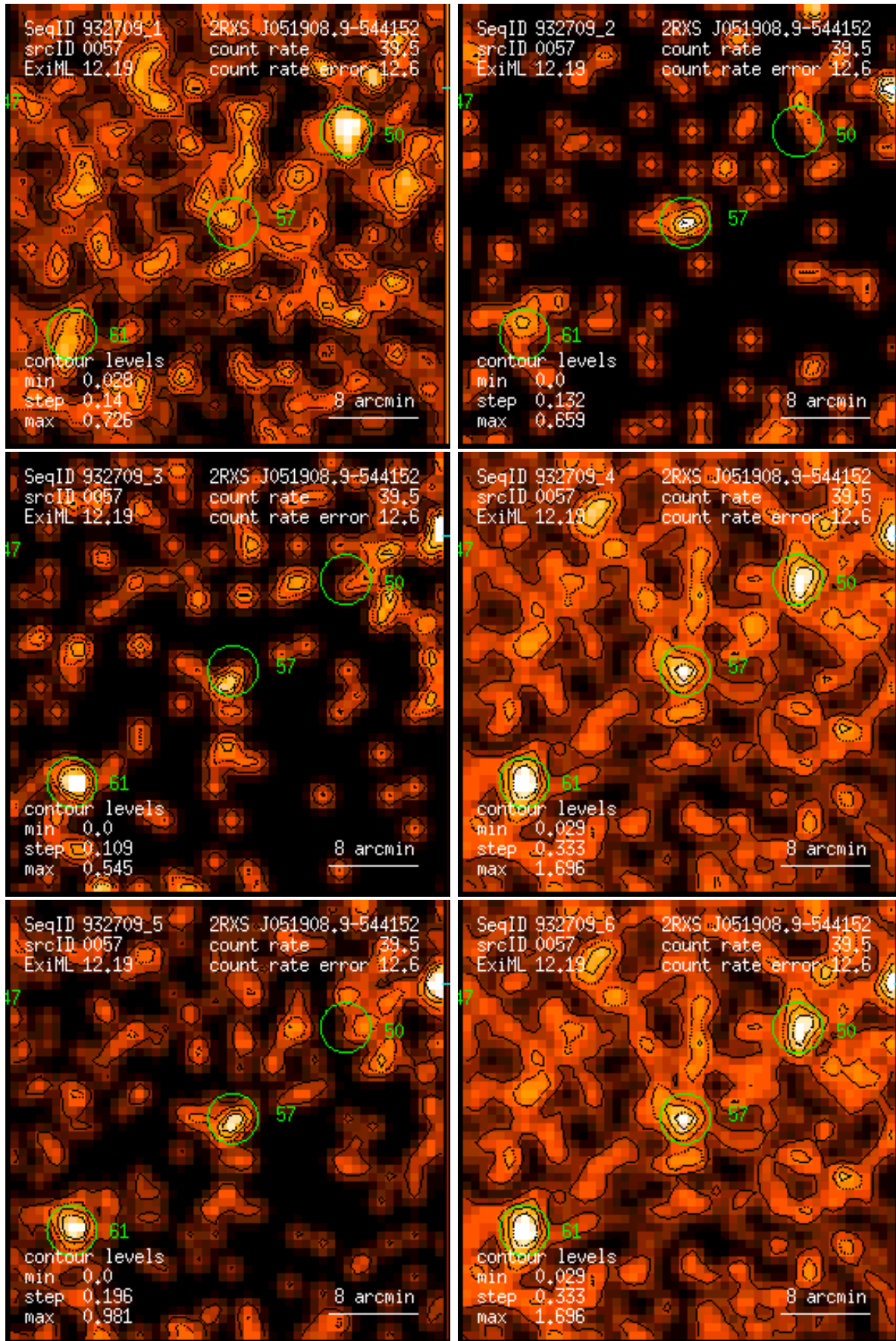
Figure 57: RASS 932709: detection 0057: band rate images, Gaussian filter: (1) PSPC channels 11 – 41, (2) 52 – 90, (3) 91 – 201, (4) 11 – 235, (5) 52 – 201, (6) 11 – 201. Broad band rates in counts/ks. Band rate contour levels in counts/ks/arcmin 2 .
