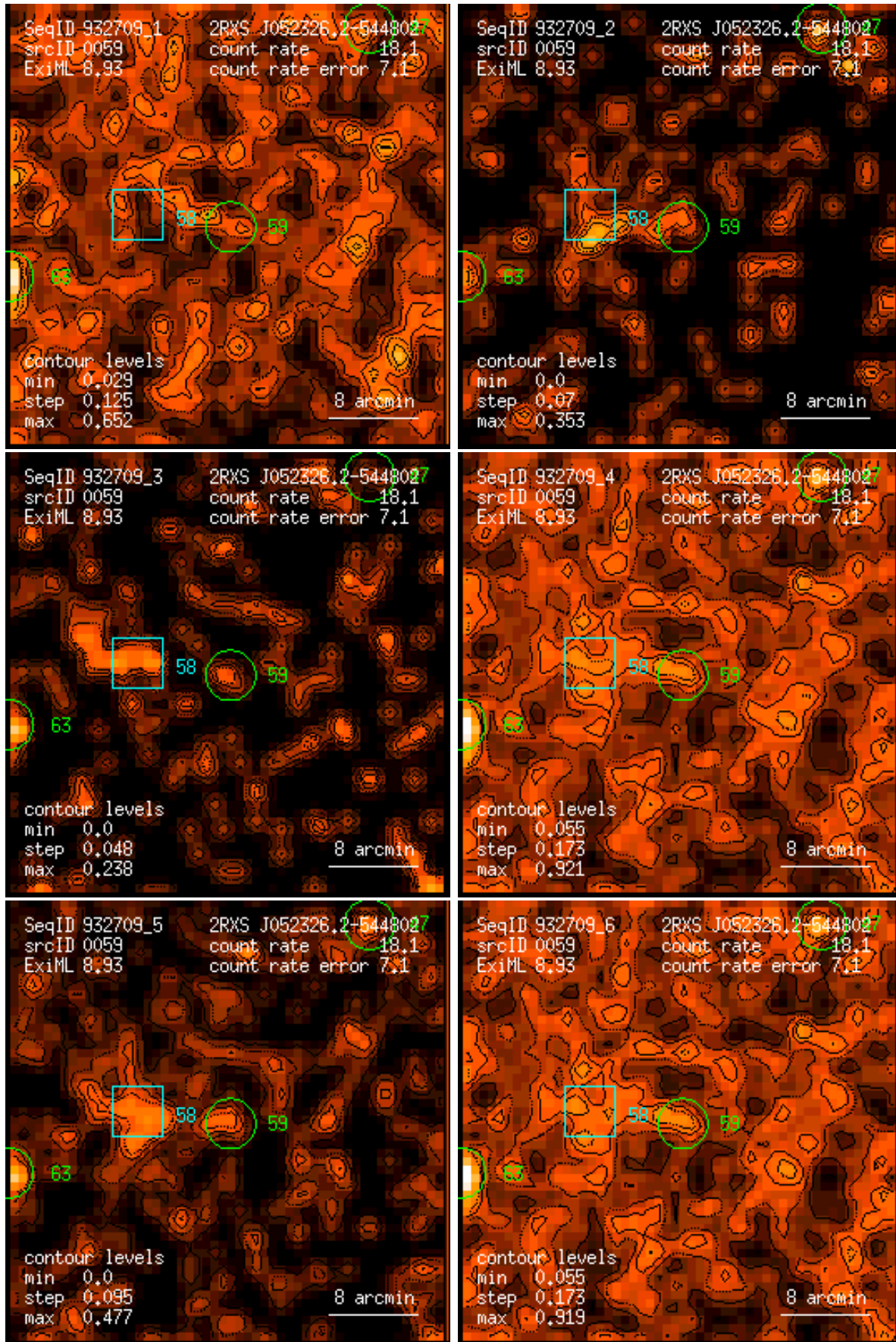
Figure 59: RASS 932709: detection 0059: band rate images, Gaussian filter: (1) PSPC channels 11 – 41, (2) 52 – 90, (3) 91 – 201, (4) 11 – 235, (5) 52 – 201, (6) 11 – 201. Broad band rates in counts/ks. Band rate contour levels in counts/ks/arcmin 2 .
