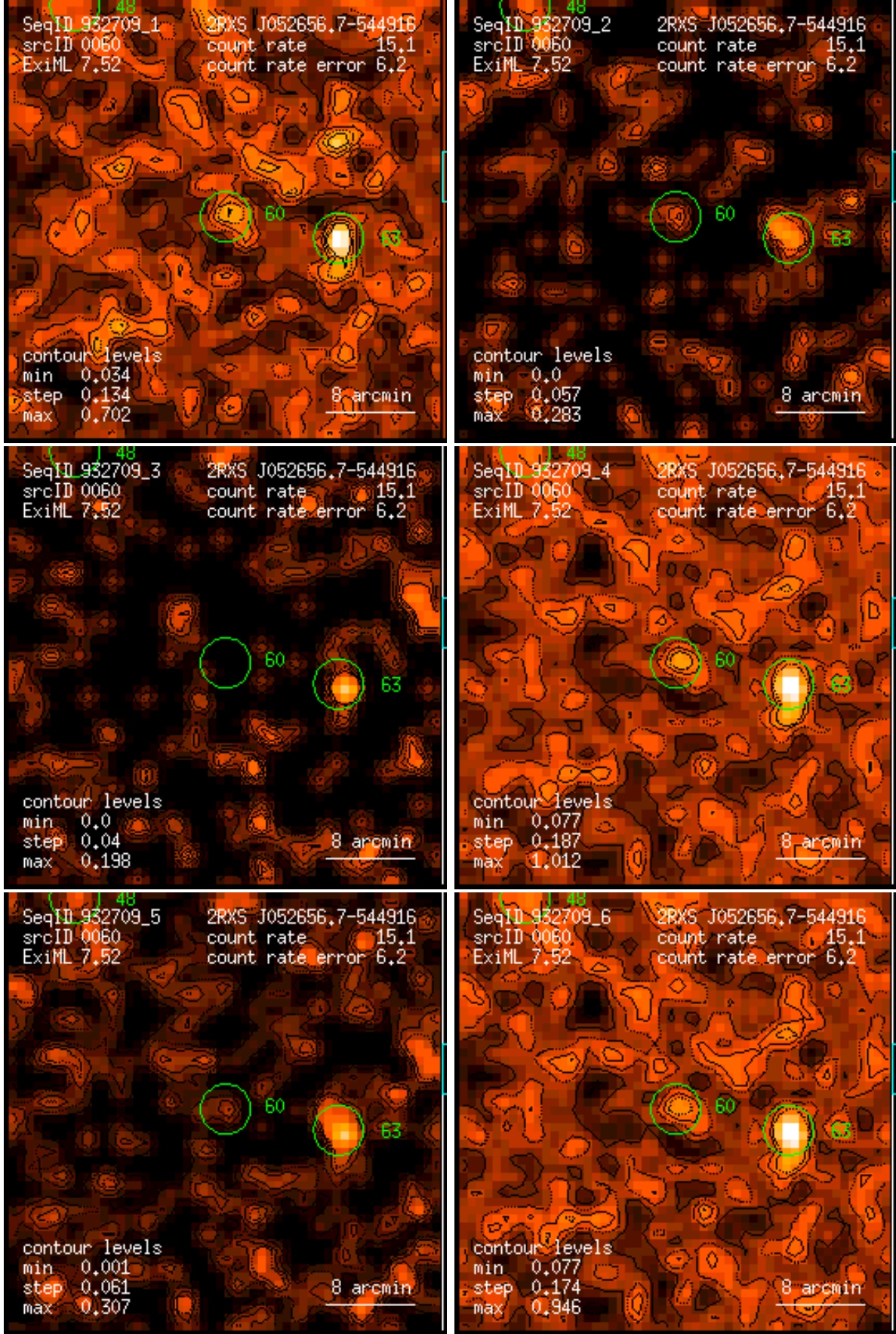
Figure 60: RASS 932709: detection 0060: band rate images, Gaussian filter: (1) PSPC channels 11 – 41, (2) 52 – 90, (3) 91 – 201, (4) 11 – 235, (5) 52 – 201, (6) 11 – 201. Broad band rates in counts/ks. Band rate contour levels in counts/ks/arcmin 2 .
