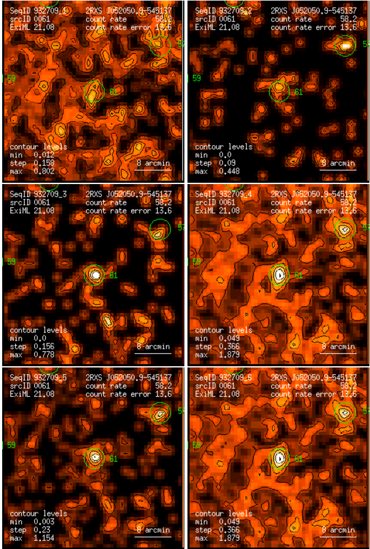
Figure 61: RASS 932709: detection 0061: band rate images, Gaussian filter: (1) PSPC channels 11 – 41, (2) 52 – 90, (3) 91 – 201, (4) 11 – 235, (5) 52 – 201, (6) 11 – 201. Broad band rates in counts/ks. Band rate contour levels in counts/ks/arcmin 2 .
