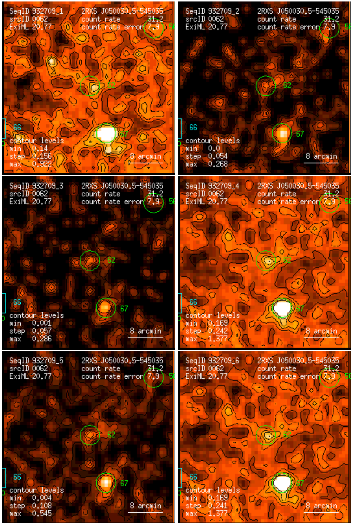
Figure 62: RASS 932709: detection 0062: band rate images, Gaussian filter: (1) PSPC channels 11 – 41, (2) 52 – 90, (3) 91 – 201, (4) 11 – 235, (5) 52 – 201, (6) 11 – 201. Broad band rates in counts/ks. Band rate contour levels in counts/ks/arcmin 2 .
