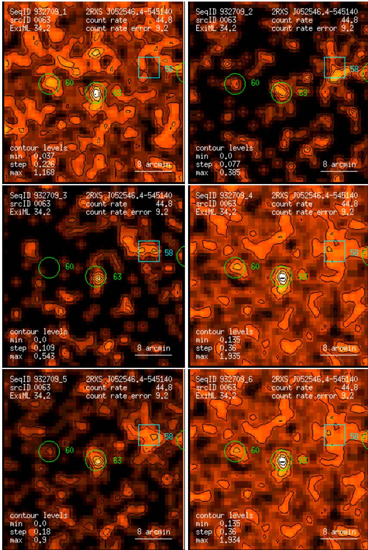
Figure 63: RASS 932709: detection 0063: band rate images, Gaussian filter: (1) PSPC channels 11 – 41, (2) 52 – 90, (3) 91 – 201, (4) 11 – 235, (5) 52 – 201, (6) 11 – 201. Broad band rates in counts/ks. Band rate contour levels in counts/ks/arcmin 2 .
