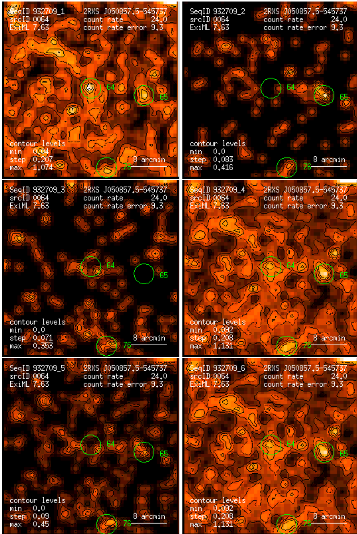
Figure 64: RASS 932709: detection 0064: band rate images, Gaussian filter: (1) PSPC channels 11 – 41, (2) 52 – 90, (3) 91 – 201, (4) 11 – 235, (5) 52 – 201, (6) 11 – 201. Broad band rates in counts/ks. Band rate contour levels in counts/ks/arcmin 2 .
