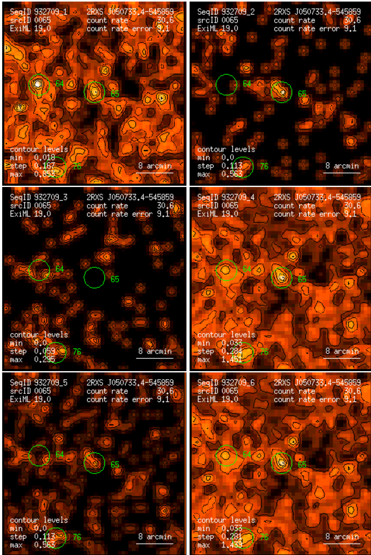
Figure 65: RASS 932709: detection 0065: band rate images, Gaussian filter: (1) PSPC channels 11 – 41, (2) 52 – 90, (3) 91 – 201, (4) 11 – 235, (5) 52 – 201, (6) 11 – 201. Broad band rates in counts/ks. Band rate contour levels in counts/ks/arcmin 2 .
