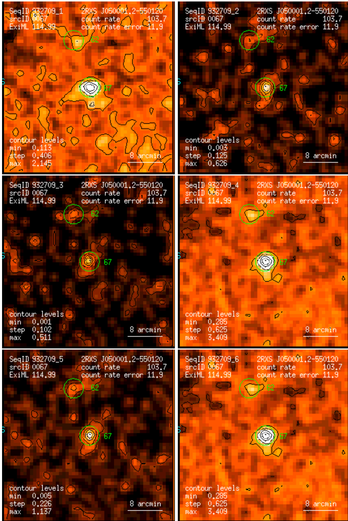
Figure 67: RASS 932709: detection 0067: band rate images, Gaussian filter: (1) PSPC channels 11 – 41, (2) 52 – 90, (3) 91 – 201, (4) 11 – 235, (5) 52 – 201, (6) 11 – 201. Broad band rates in counts/ks. Band rate contour levels in counts/ks/arcmin 2 .
