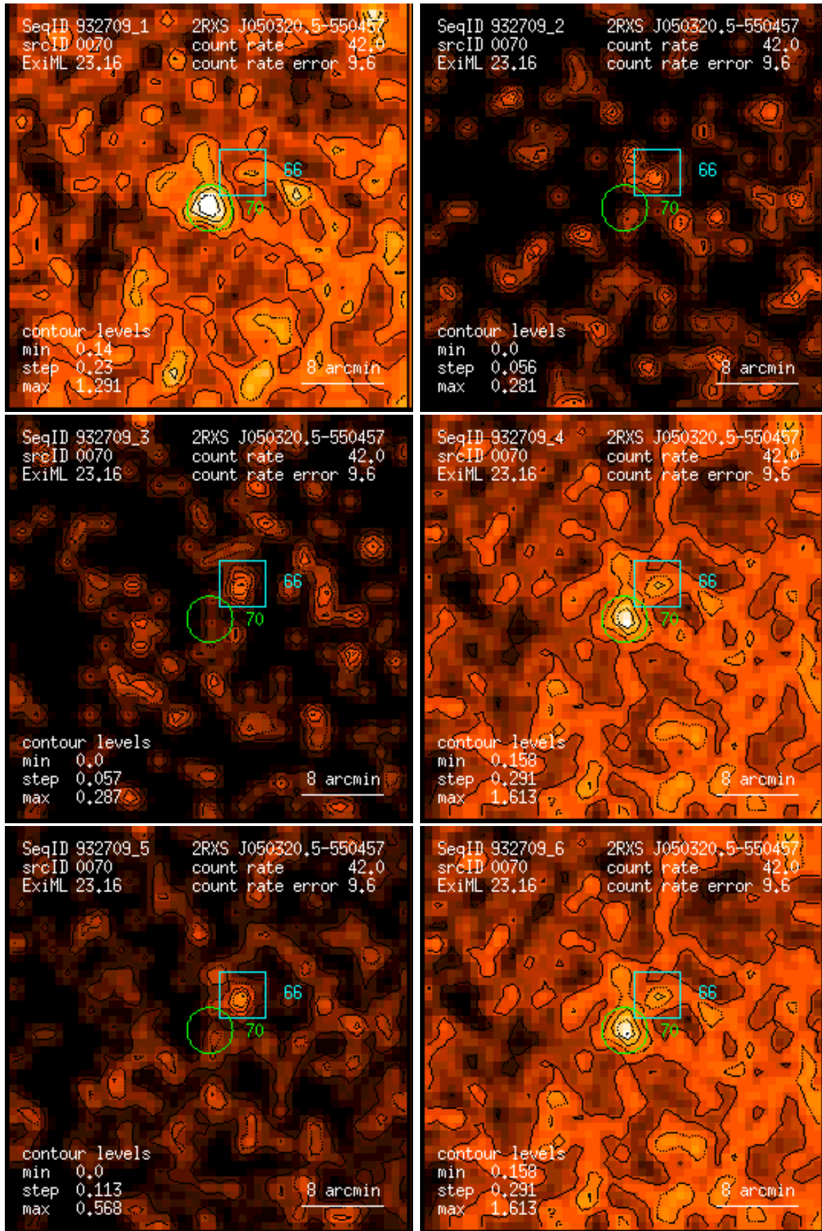
Figure 70: RASS 932709: detection 0070: band rate images, Gaussian filter: (1) PSPC channels 11 – 41, (2) 52 – 90, (3) 91 – 201, (4) 11 – 235, (5) 52 – 201, (6) 11 – 201. Broad band rates in counts/ks. Band rate contour levels in counts/ks/arcmin 2 .
