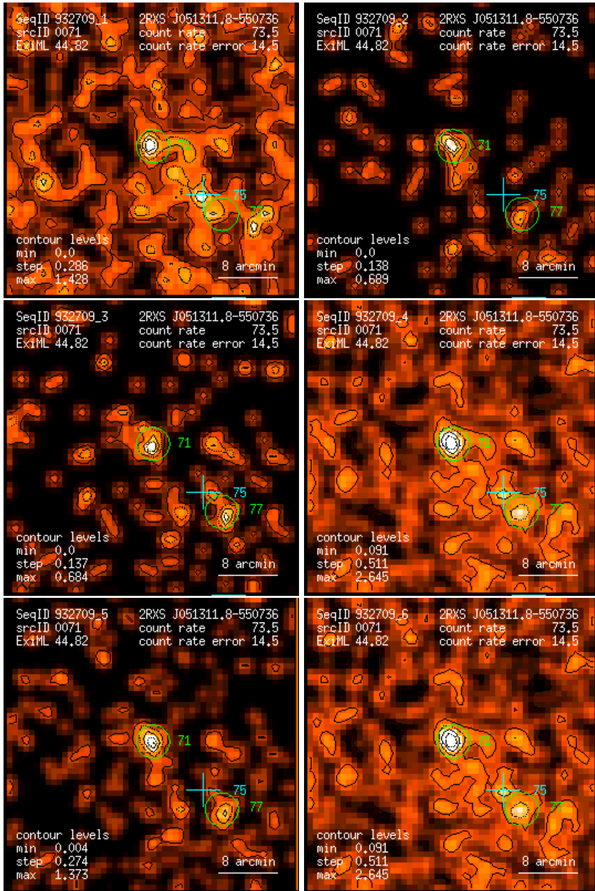
Figure 71: RASS 932709: detection 0071: band rate images, Gaussian filter: (1) PSPC channels 11 – 41, (2) 52 – 90, (3) 91 – 201, (4) 11 – 235, (5) 52 – 201, (6) 11 – 201. Broad band rates in counts/ks. Band rate contour levels in counts/ks/arcmin 2 .
