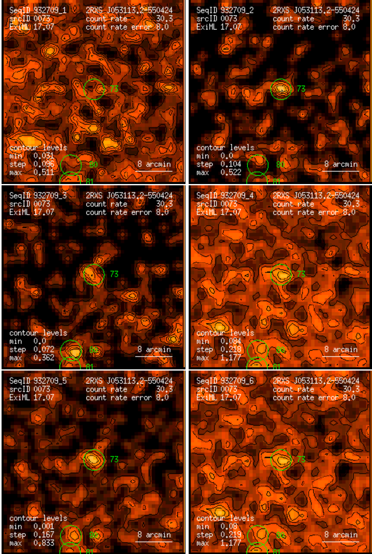
Figure 73: RASS 932709: detection 0073: band rate images, Gaussian filter: (1) PSPC channels 11 – 41, (2) 52 – 90, (3) 91 – 201, (4) 11 – 235, (5) 52 – 201, (6) 11 – 201. Broad band rates in counts/ks. Band rate contour levels in counts/ks/arcmin 2 .
