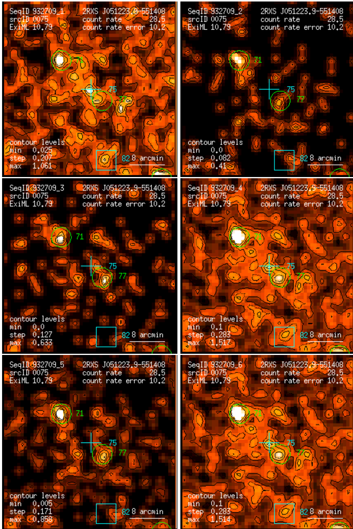
Figure 75: RASS 932709: detection 0075: band rate images, Gaussian filter: (1) PSPP channels 11 – 41, (2) 52 – 90, (3) 91 – 201, (4) 11 – 235, (5) 52 – 201, (6) 11 – 201. Broad band rates in counts/ks. Band rate contour levels in counts/ks/arcmin 2 .
