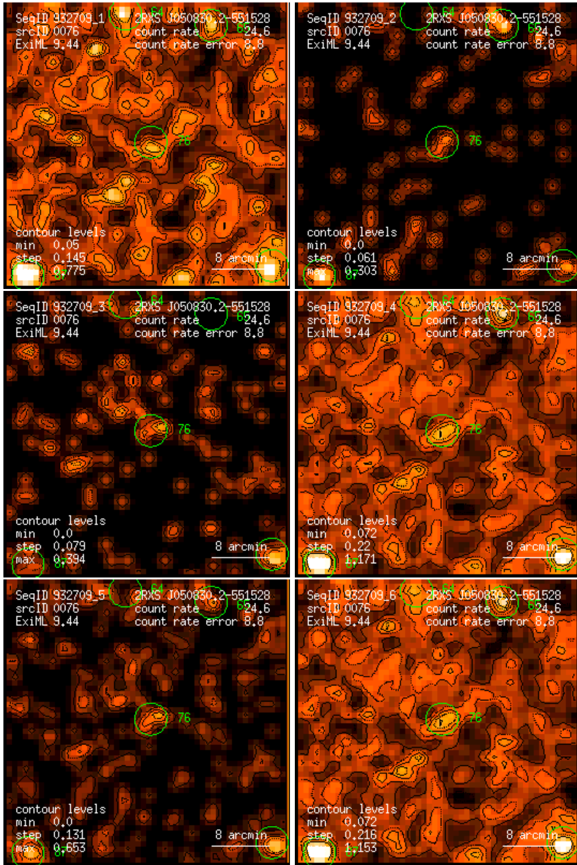
Figure 76: RASS 932709: detection 0076: band rate images, Gaussian filter: (1) PSPC channels 11 – 41, (2) 52 – 90, (3) 91 – 201, (4) 11 – 235, (5) 52 – 201, (6) 11 – 201. Broad band rates in counts/ks. Band rate contour levels in counts/ks/arcmin 2 .
