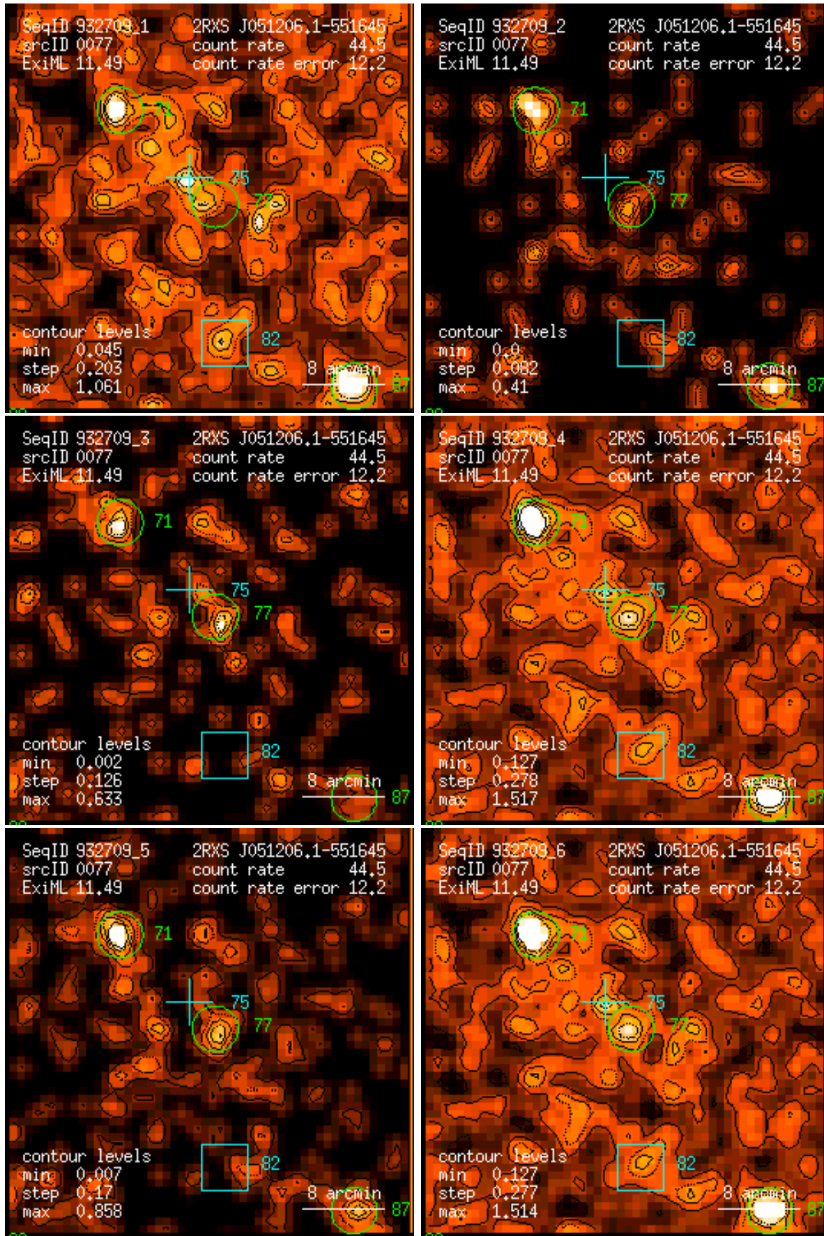
Figure 77: RASS 932709: detection 0077: band rate images, Gaussian filter: (1) PSPC channels 11 – 41, (2) 52 – 90, (3) 91 – 201, (4) 11 – 235, (5) 52 – 201, (6) 11 – 201. Broad band rates in counts/ks. Band rate contour levels in counts/ks/arcmin 2 .
