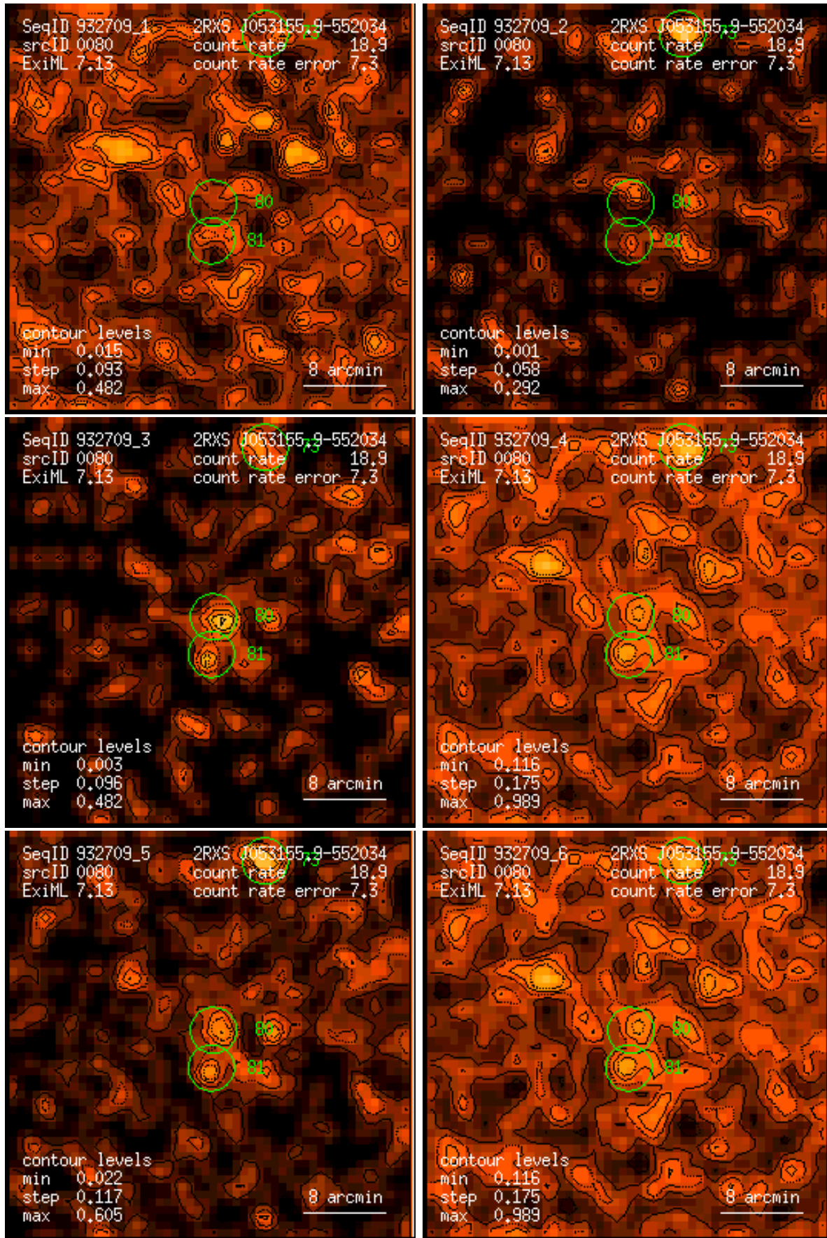
Figure 80: RASS 932709: detection 0080: band rate images, Gaussian filter: (1) PSPC channels 11 – 41, (2) 52 – 90, (3) 91 – 201, (4) 11 – 235, (5) 52 – 201, (6) 11 – 201. Broad band rates in counts/ks. Band rate contour levels in counts/ks/arcmin 2 .
