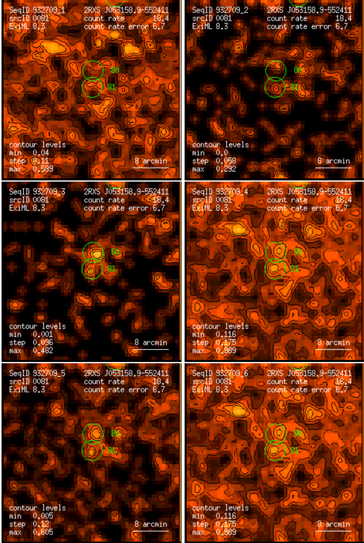
Figure 81: RASS 932709: detection 0081: band rate images, Gaussian filter: (1) PSPC channels 11 – 41, (2) 52 – 90, (3) 91 – 201, (4) 11 – 235, (5) 52 – 201, (6) 11 – 201. Broad band rates in counts/ks. Band rate contour levels in counts/ks/arcmin 2 .
