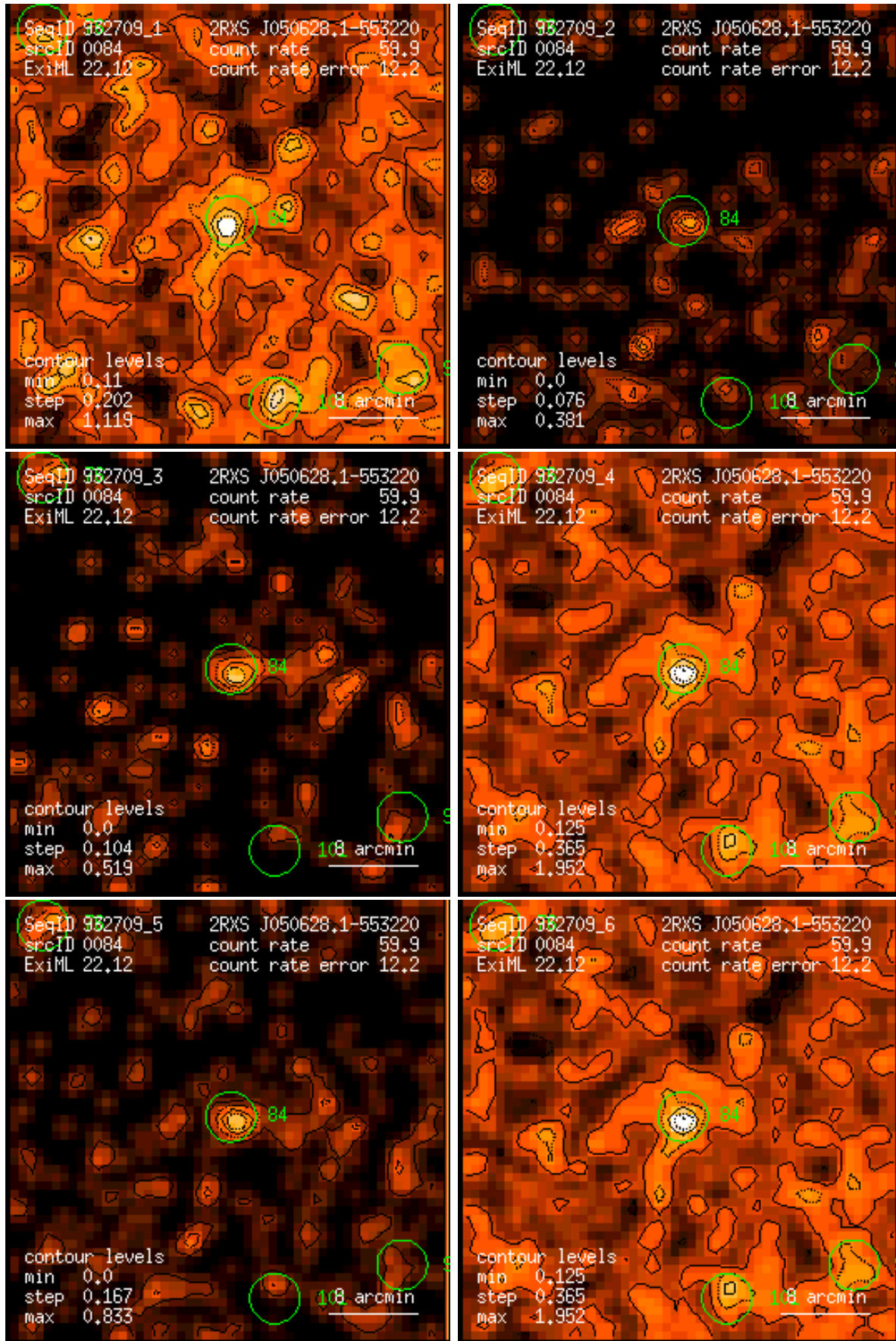
Figure 84: RASS 932709: detection 0084: band rate images, Gaussian filter: (1) PSPC channels 11 – 41, (2) 52 – 90, (3) 91 – 201, (4) 11 – 235, (5) 52 – 201, (6) 11 – 201. Broad band rates in counts/ks. Band rate contour levels in counts/ks/arcmin 2 .
