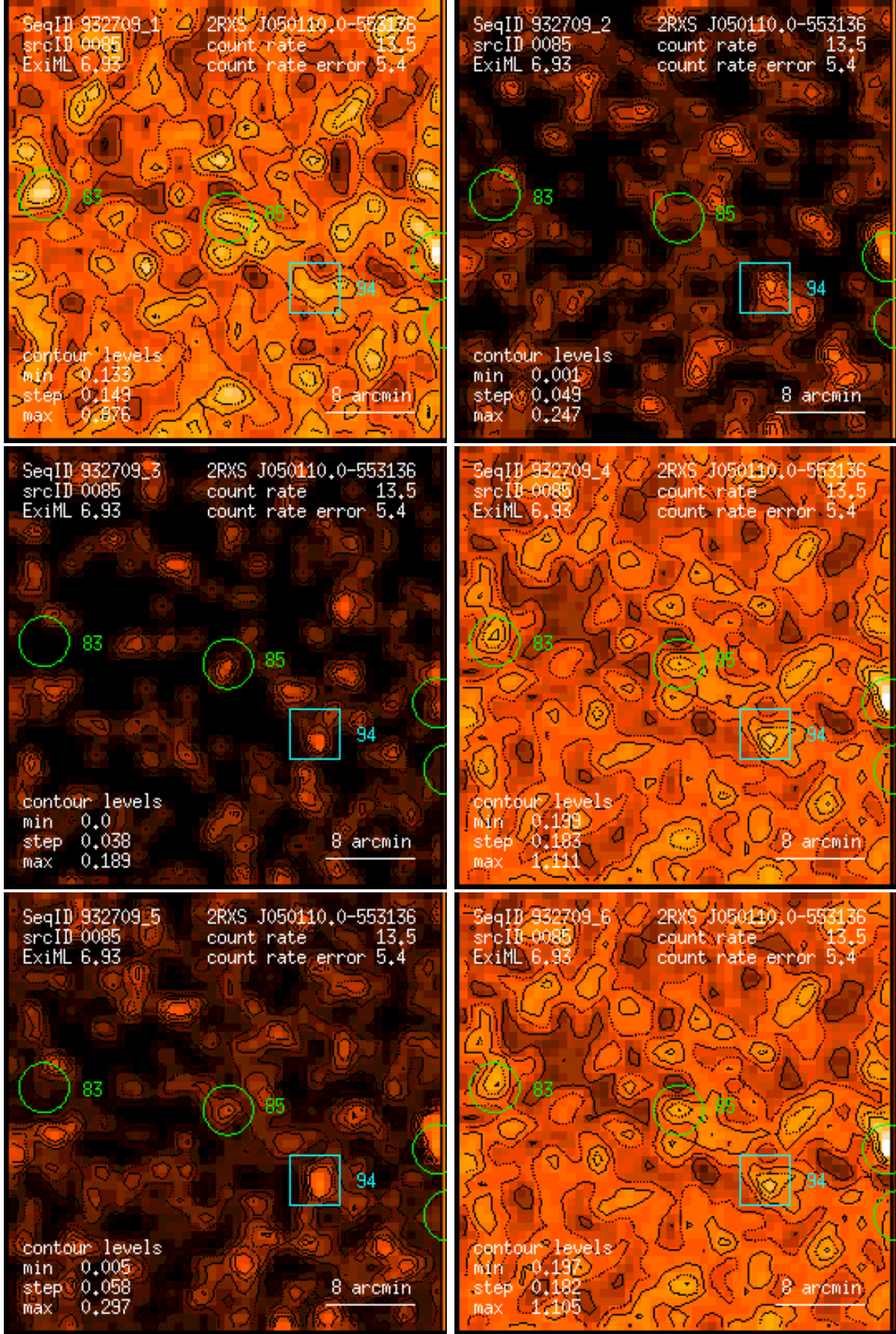
Figure 85: RASS 932709: detection 0085: band rate images, Gaussian filter: (1) PSPC channels 11 – 41, (2) 52 – 90, (3) 91 – 201, (4) 11 – 235, (5) 52 – 201, (6) 11 – 201. Broad band rates in counts/ks. Band rate contour levels in counts/ks/arcmin 2 .
