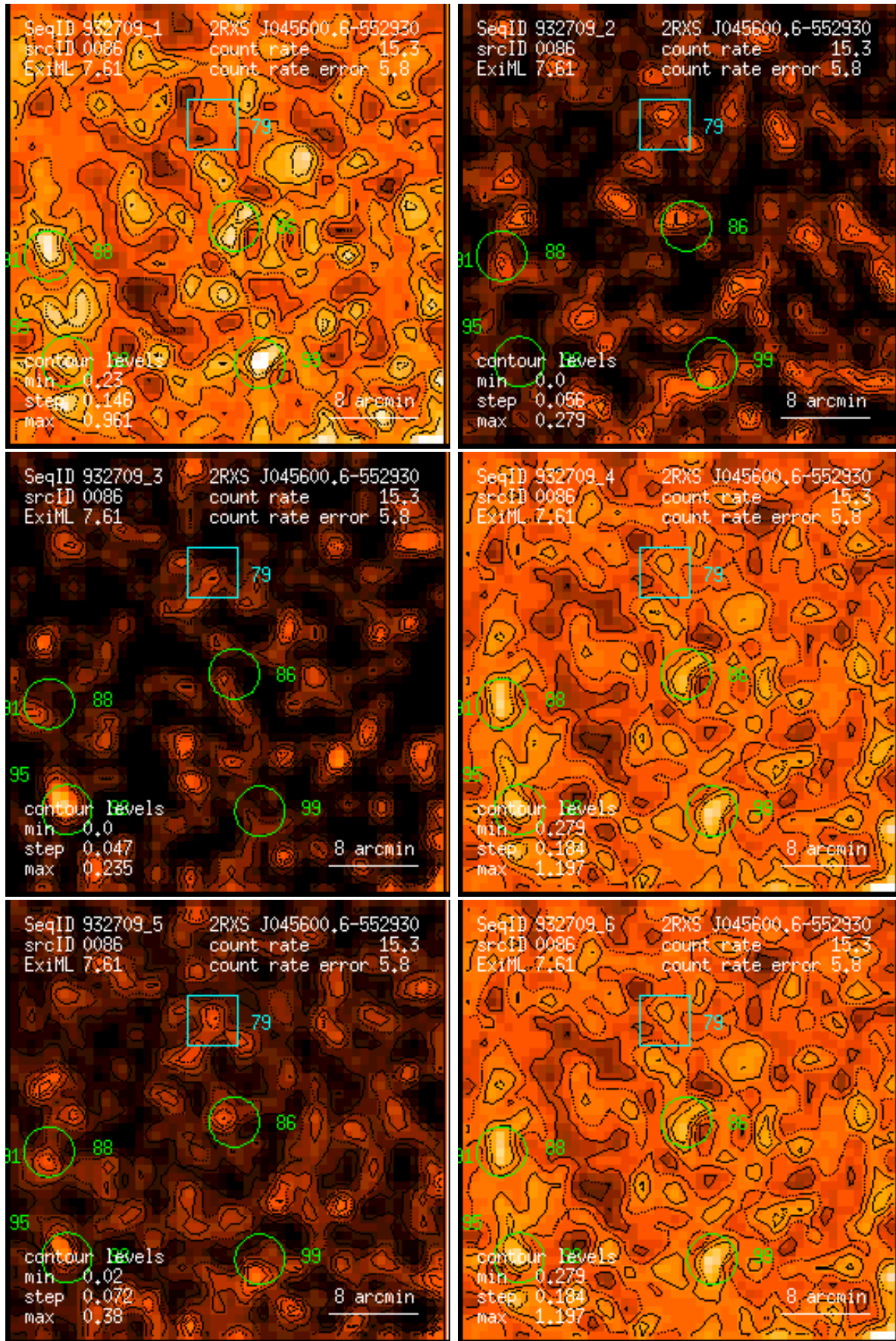
Figure 86: RASS 932709: detection 0086: band rate images, Gaussian filter: (1) PSPC channels 11 – 41, (2) 52 – 90, (3) 91 – 201, (4) 11 – 235, (5) 52 – 201, (6) 11 – 201. Broad band rates in counts/ks. Band rate contour levels in counts/ks/arcmin 2 .
