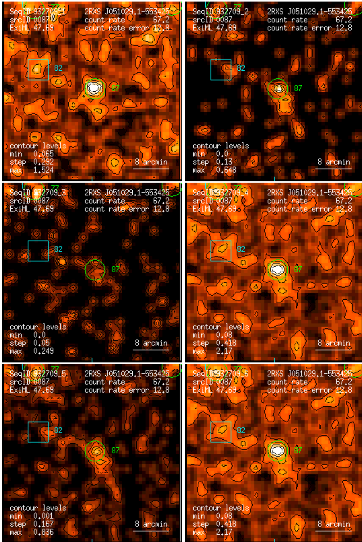
Figure 87: RASS 932709: detection 0087: band rate images, Gaussian filter: (1) PSPC channels 11 – 41, (2) 52 – 90, (3) 91 – 201, (4) 11 – 235, (5) 52 – 201, (6) 11 – 201. Broad band rates in counts/ks. Band rate contour levels in counts/ks/arcmin 2 .
