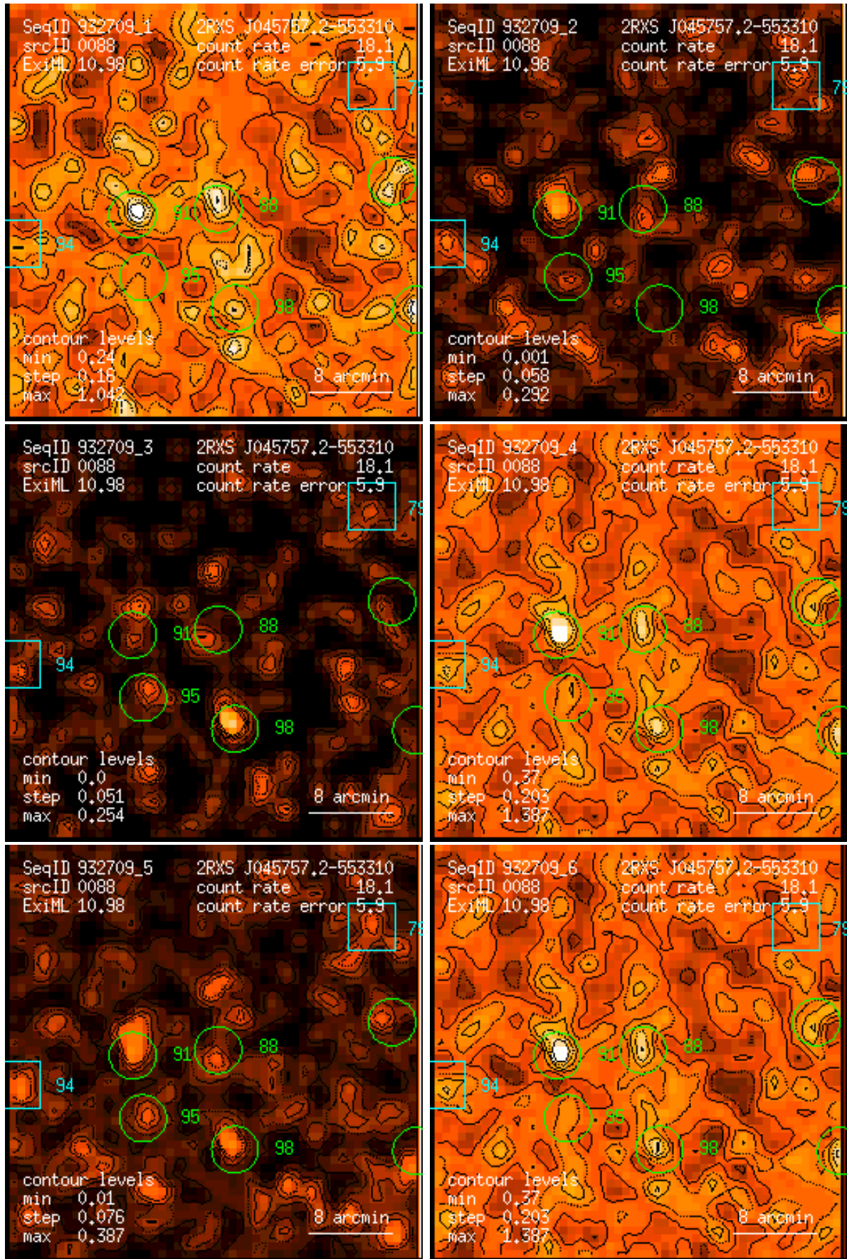
Figure 88: RASS 932709: detection 0088: band rate images, Gaussian filter: (1) PSPC channels 11 – 41, (2) 52 – 90, (3) 91 – 201, (4) 11 – 235, (5) 52 – 201, (6) 11 – 201. Broad band rates in counts/ks. Band rate contour levels in counts/ks/arcmin 2 .
