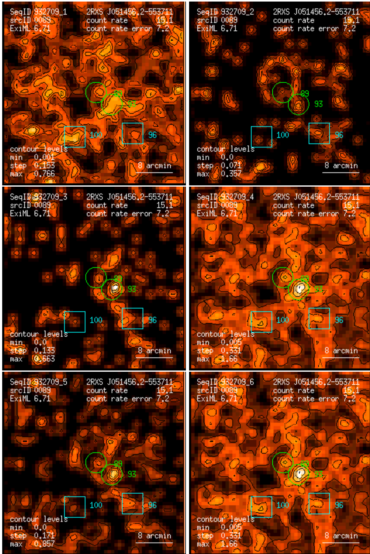
Figure 89: RASS 932709: detection 0089: band rate images, Gaussian filter: (1) PSPC channels 11 – 41, (2) 52 – 90, (3) 91 – 201, (4) 11 – 235, (5) 52 – 201, (6) 11 – 201. Broad band rates in counts/ks. Band rate contour levels in counts/ks/arcmin 2 .
