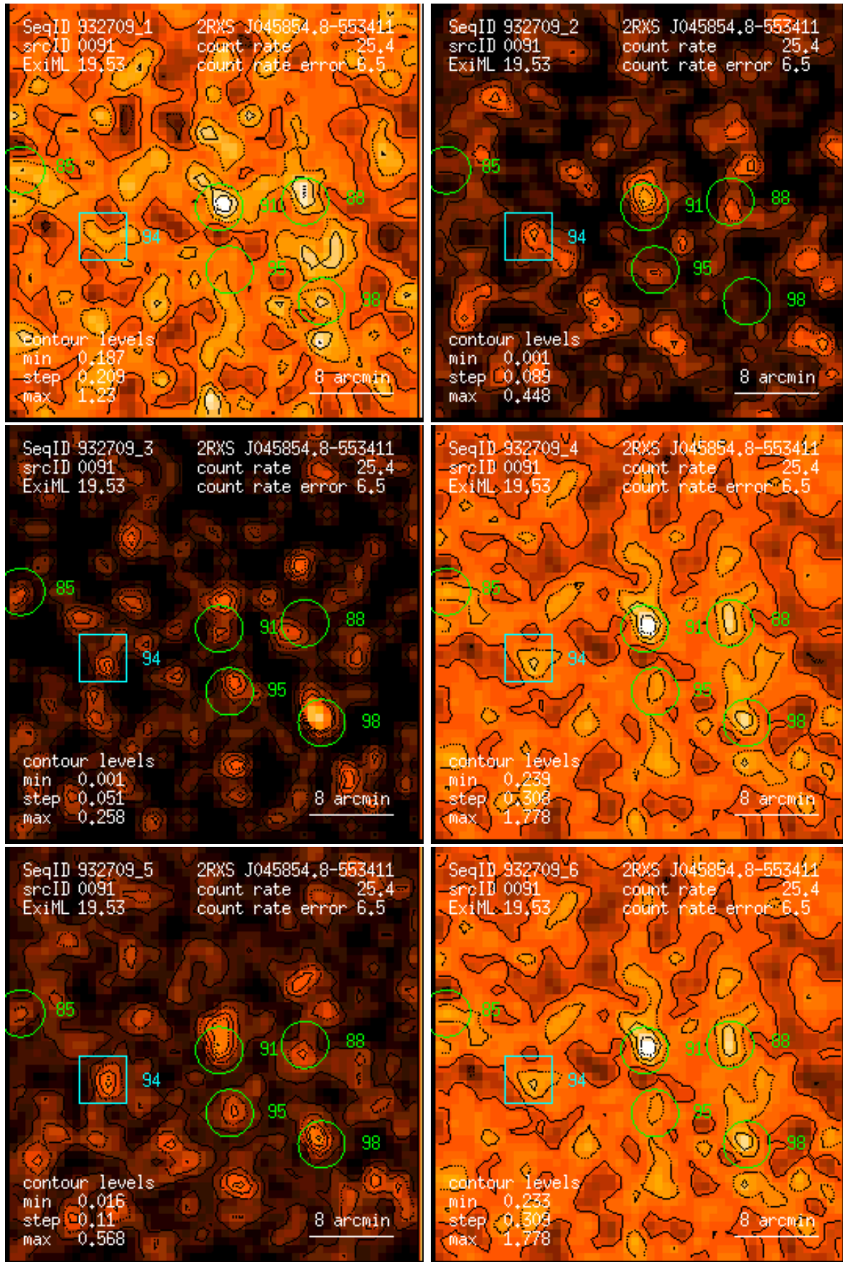
Figure 91: RASS 932709: detection 0091: band rate images, Gaussian filter: (1) PSPC channels 11 – 41, (2) 52 – 90, (3) 91 – 201, (4) 11 – 235, (5) 52 – 201, (6) 11 – 201. Broad band rates in counts/ks. Band rate contour levels in counts/ks/arcmin 2 .
