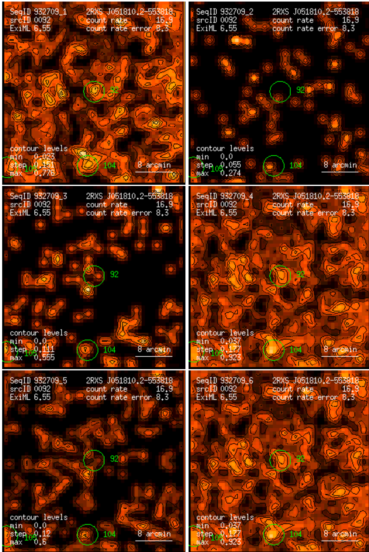
Figure 92: RASS 932709: detection 0092: band rate images, Gaussian filter: (1) PSPC channels 11 – 41, (2) 52 – 90, (3) 91 – 201, (4) 11 – 235, (5) 52 – 201, (6) 11 – 201. Broad band rates in counts/ks. Band rate contour levels in counts/ks/arcmin 2 .
