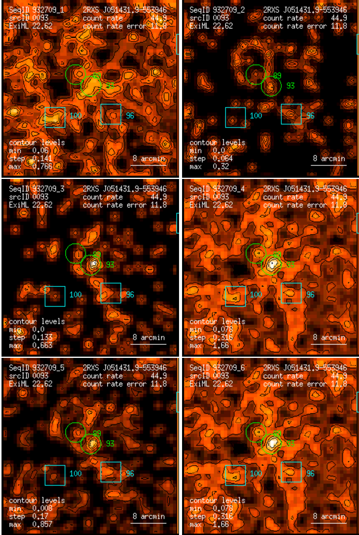
Figure 93: RASS 932709: detection 0093: band rate images, Gaussian filter: (1) PSPC channels 11 – 41, (2) 52 – 90, (3) 91 – 201, (4) 11 – 235, (5) 52 – 201, (6) 11 – 201. Broad band rates in counts/ks. Band rate contour levels in counts/ks/arcmin 2 .
