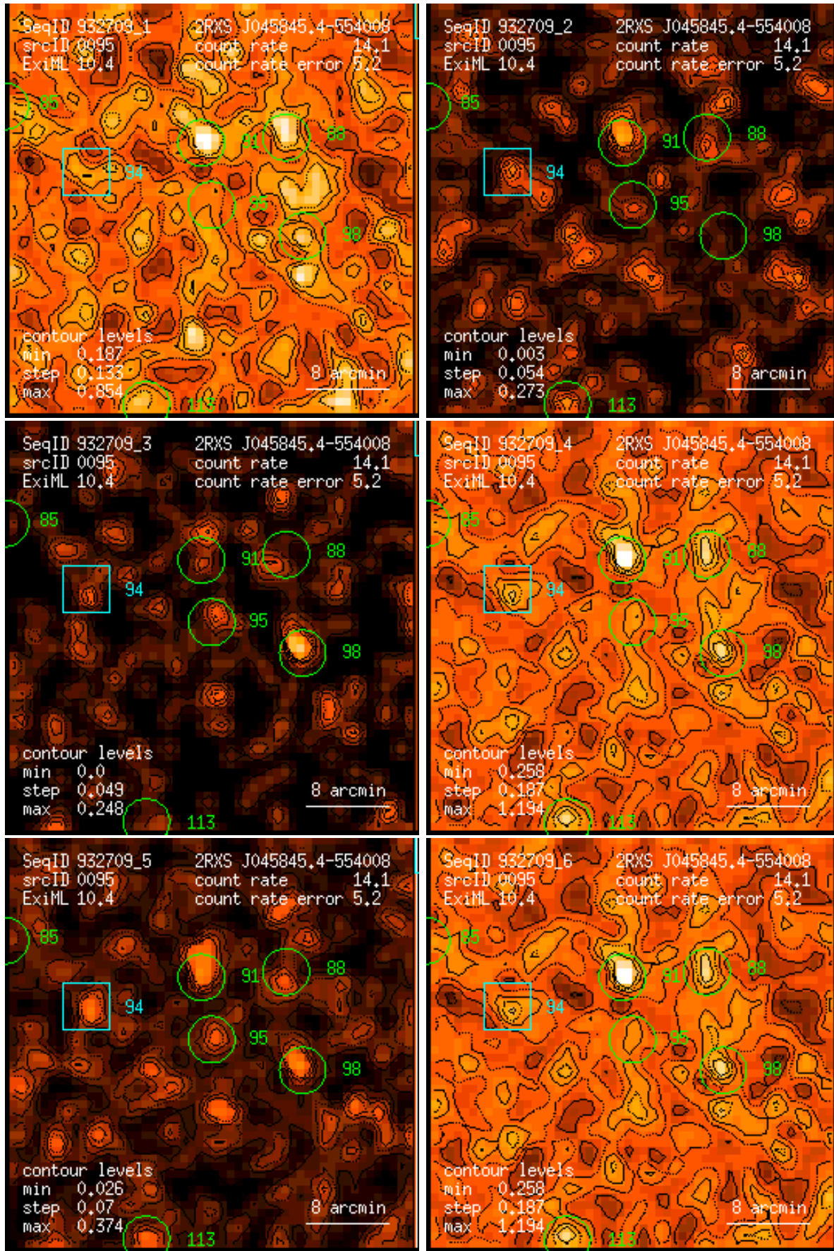
Figure 95: RASS 932709: detection 0095: band rate images, Gaussian filter: (1) PSPC channels 11 – 41, (2) 52 – 90, (3) 91 – 201, (4) 11 – 235, (5) 52 – 201, (6) 11 – 201. Broad band rates in counts/ks. Band rate contour levels in counts/ks/arcmin 2 .
