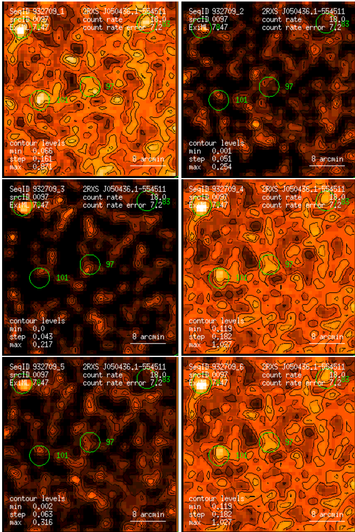
Figure 97: RASS 932709: detection 0097: band rate images, Gaussian filter: (1) PSPC channels 11 – 41, (2) 52 – 90, (3) 91 – 201, (4) 11 – 235, (5) 52 – 201, (6) 11 – 201. Broad band rates in counts/ks. Band rate contour levels in counts/ks/arcmin 2 .
