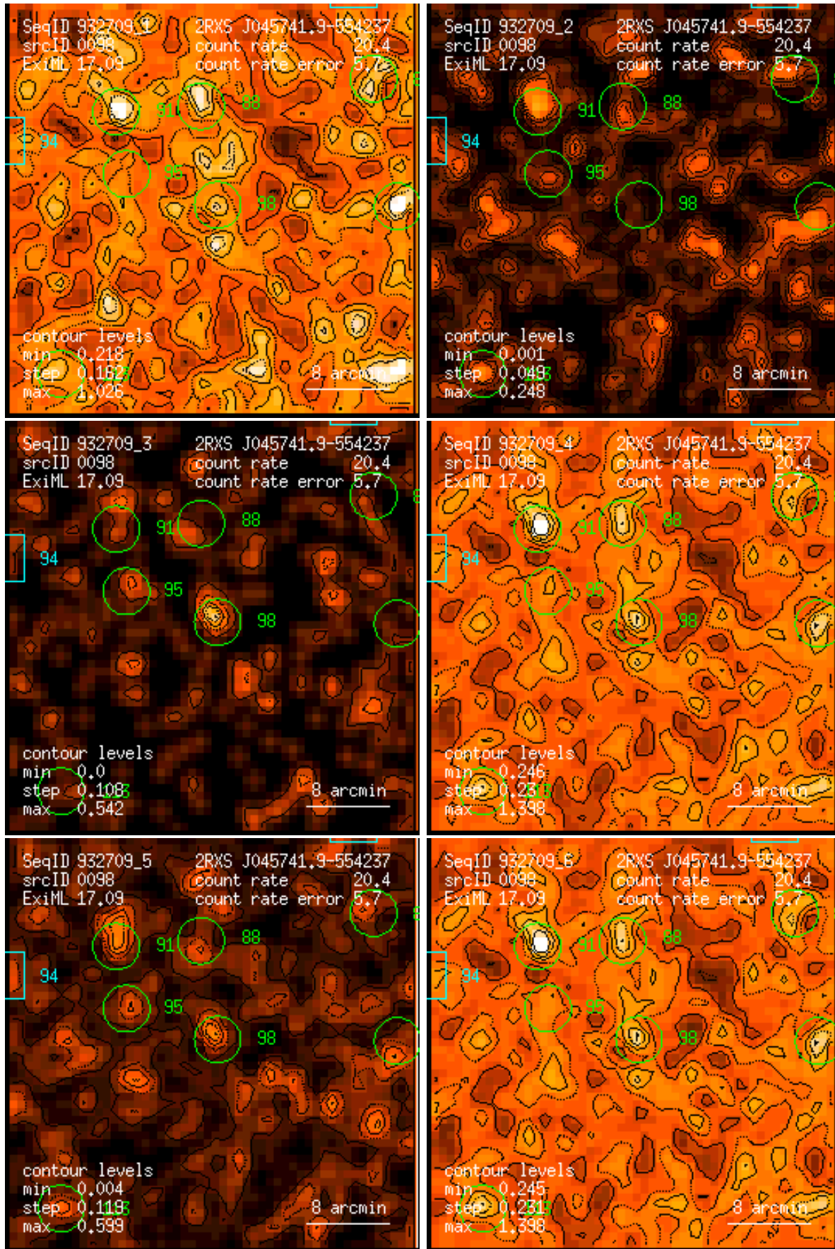
Figure 98: RASS 932709: detection 0098: band rate images, Gaussian filter: (1) PSPC channels 11 – 41, (2) 52 – 90, (3) 91 – 201, (4) 11 – 235, (5) 52 – 201, (6) 11 – 201. Broad band rates in counts/ks. Band rate contour levels in counts/ks/arcmin 2 .
