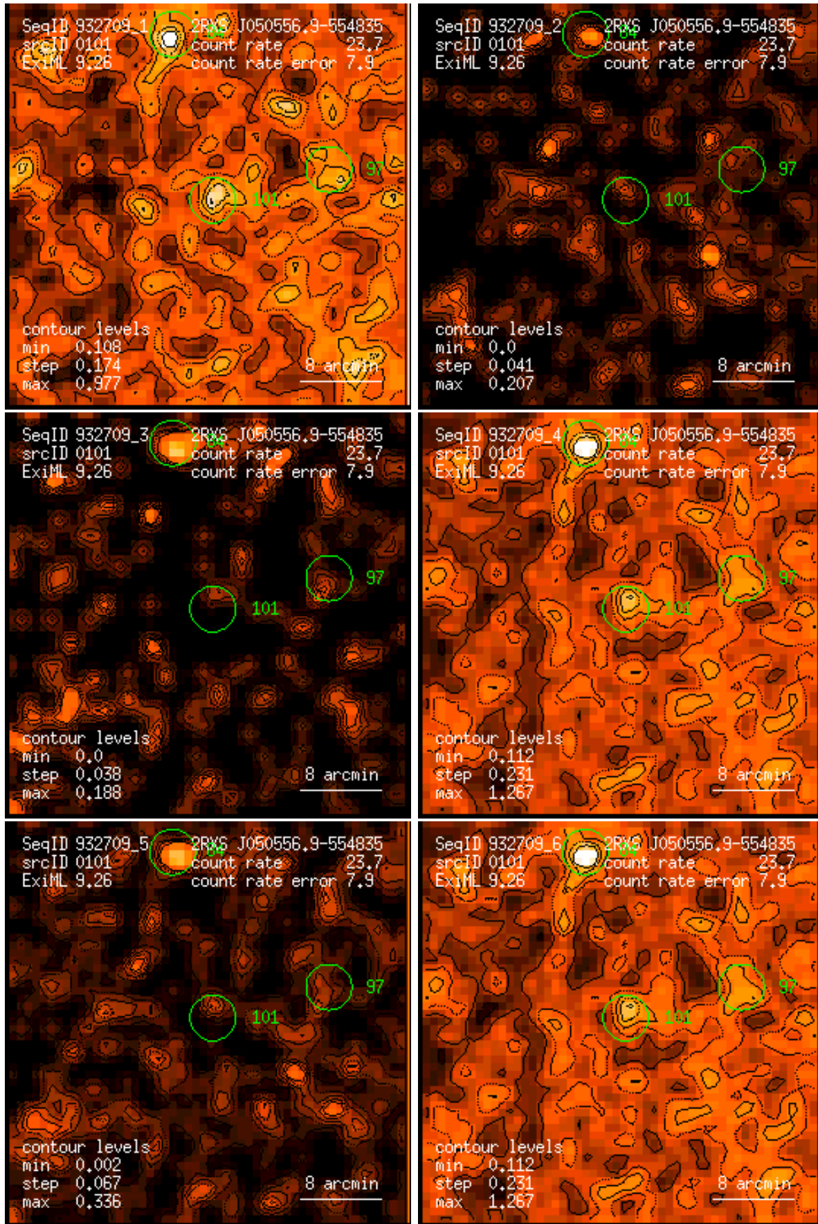
Figure 101: RASS 932709: detection 0101: band rate images, Gaussian filter: (1) PSPC channels 11 – 41, (2) 52 – 90, (3) 91 – 201, (4) 11 – 235, (5) 52 – 201, (6) 11 – 201. Broad band rates in counts/ks. Band rate contour levels in counts/ks/arcmin 2 .
