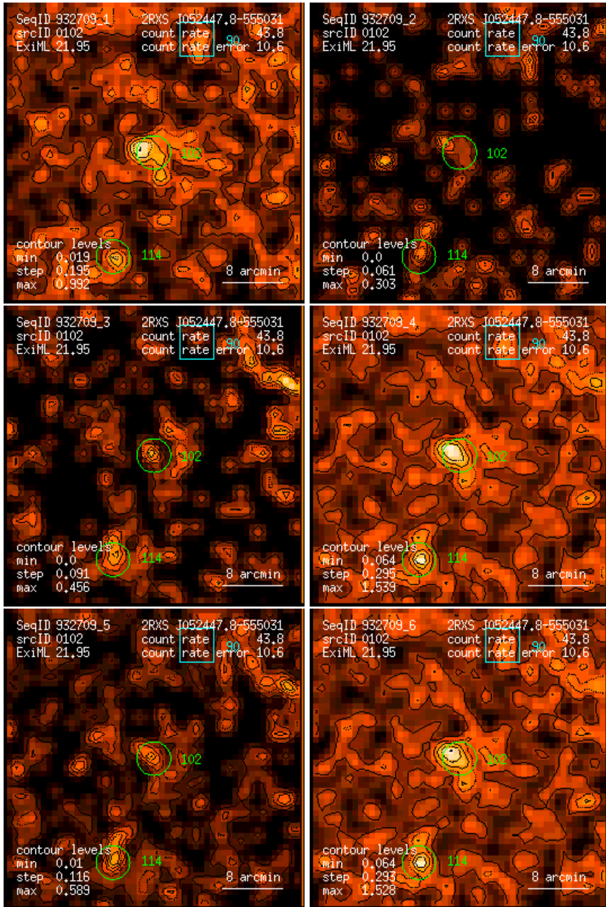
Figure 102: RASS 932709: detection 0102: band rate images, Gaussian filter: (1) PSPC channels 11 – 41, (2) 52 – 90, (3) 91 – 201, (4) 11 – 235, (5) 52 – 201, (6) 11 – 201. Broad band rates in counts/ks. Band rate contour levels in counts/ks/arcmin 2 .
