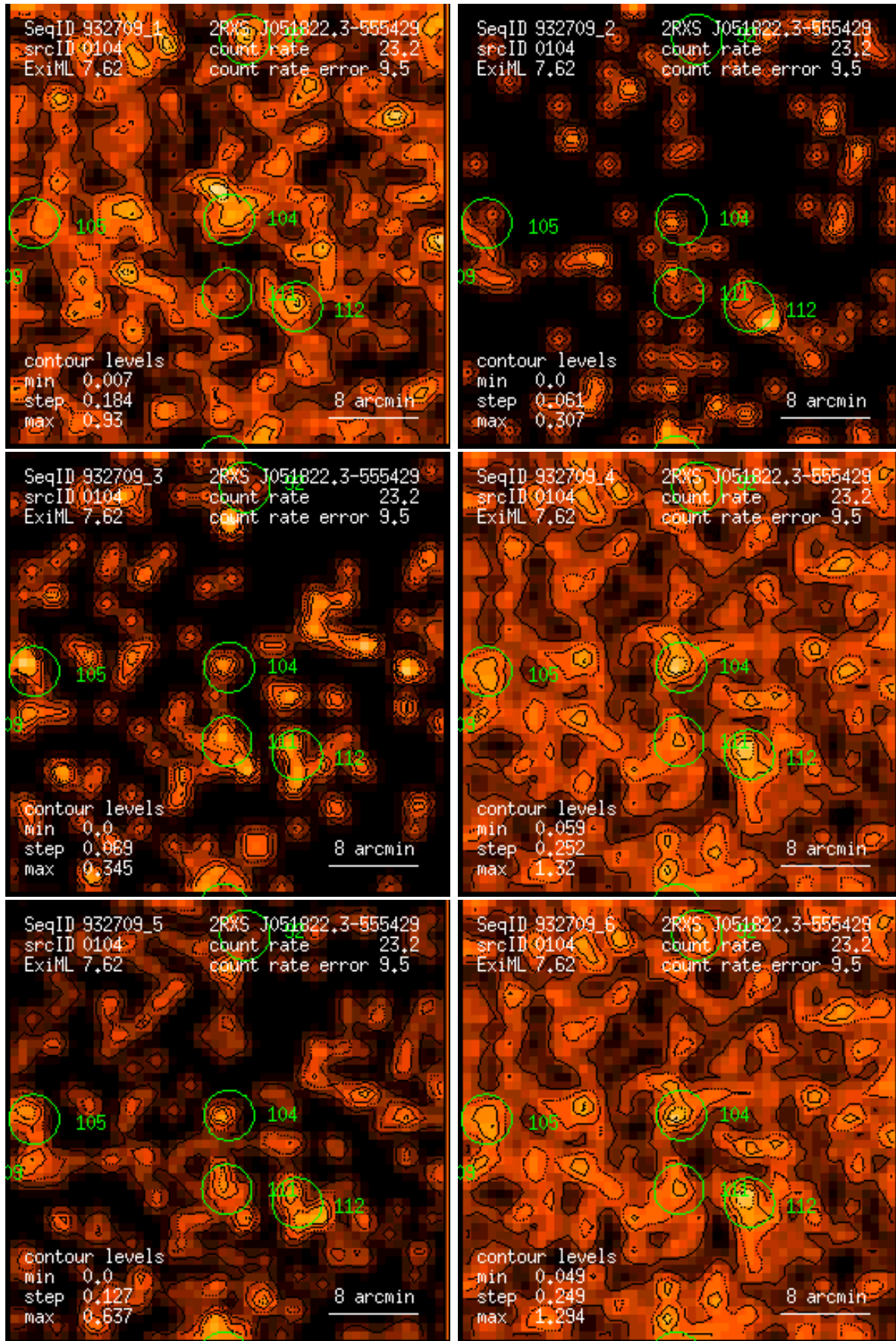
Figure 104: RASS 932709: detection 0104: band rate images, Gaussian filter: (1) PSPC channels 11 – 41, (2) 52 – 90, (3) 91 – 201, (4) 11 – 235, (5) 52 – 201, (6) 11 – 201. Broad band rates in counts/ks. Band rate contour levels in counts/ks/arcmin 2 .
