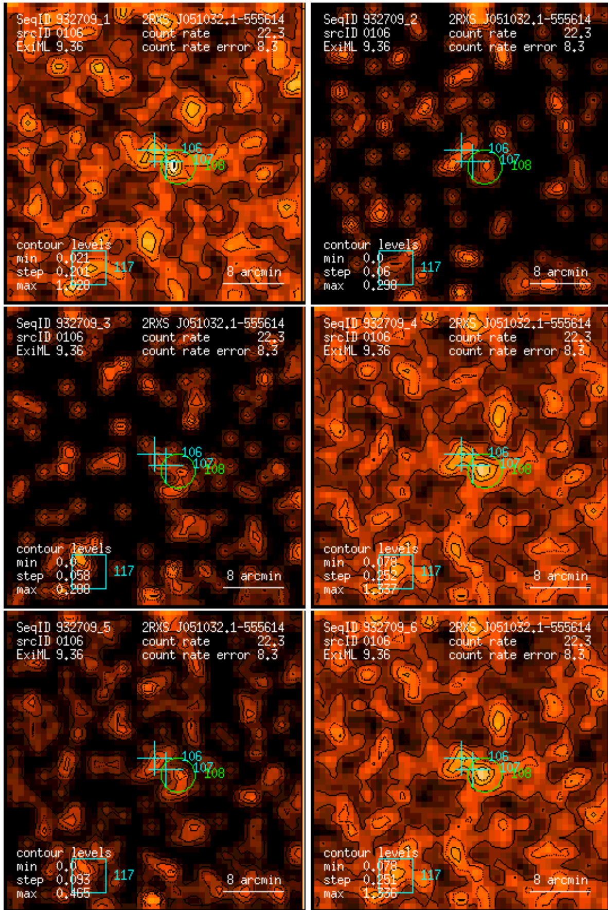
Figure 106: RASS 932709: detection 0106: band rate images, Gaussian filter: (1) PSPC channels 11 – 41, (2) 52 – 90, (3) 91 – 201, (4) 11 – 235, (5) 52 – 201, (6) 11 – 201. Broad band rates in counts/ks. Band rate contour levels in counts/ks/arcmin 2 .
