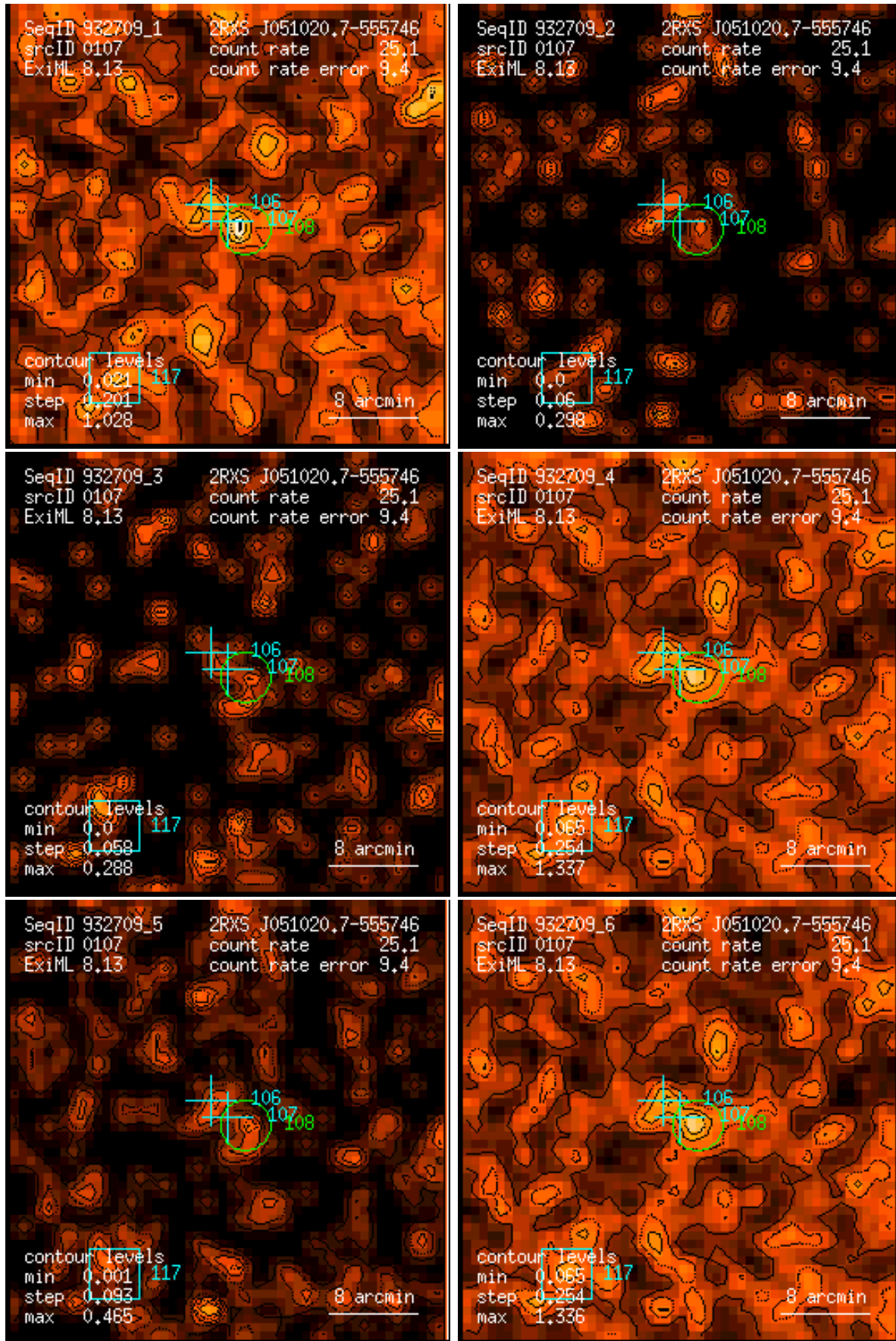
Figure 107: RASS 932709: detection 0107: band rate images, Gaussian filter: (1) PSPC channels 11 – 41, (2) 52 – 90, (3) 91 – 201, (4) 11 – 235, (5) 52 – 201, (6) 11 – 201. Broad band rates in counts/ks. Band rate contour levels in counts/ks/arcmin 2 .
