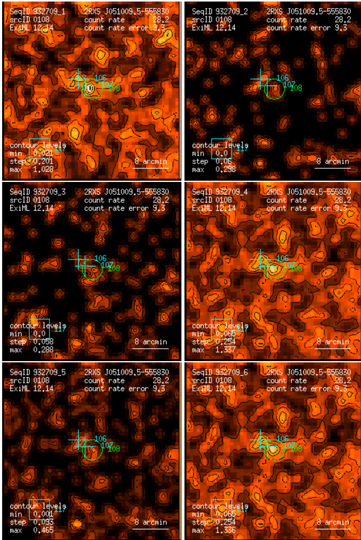
Figure 108: RASS 932709: detection 0108: band rate images, Gaussian filter: (1) PSPC channels 11 – 41, (2) 52 – 90, (3) 91 – 201, (4) 11 – 235, (5) 52 – 201, (6) 11 – 201. Broad band rates in counts/ks. Band rate contour levels in counts/ks/arcmin 2 .
