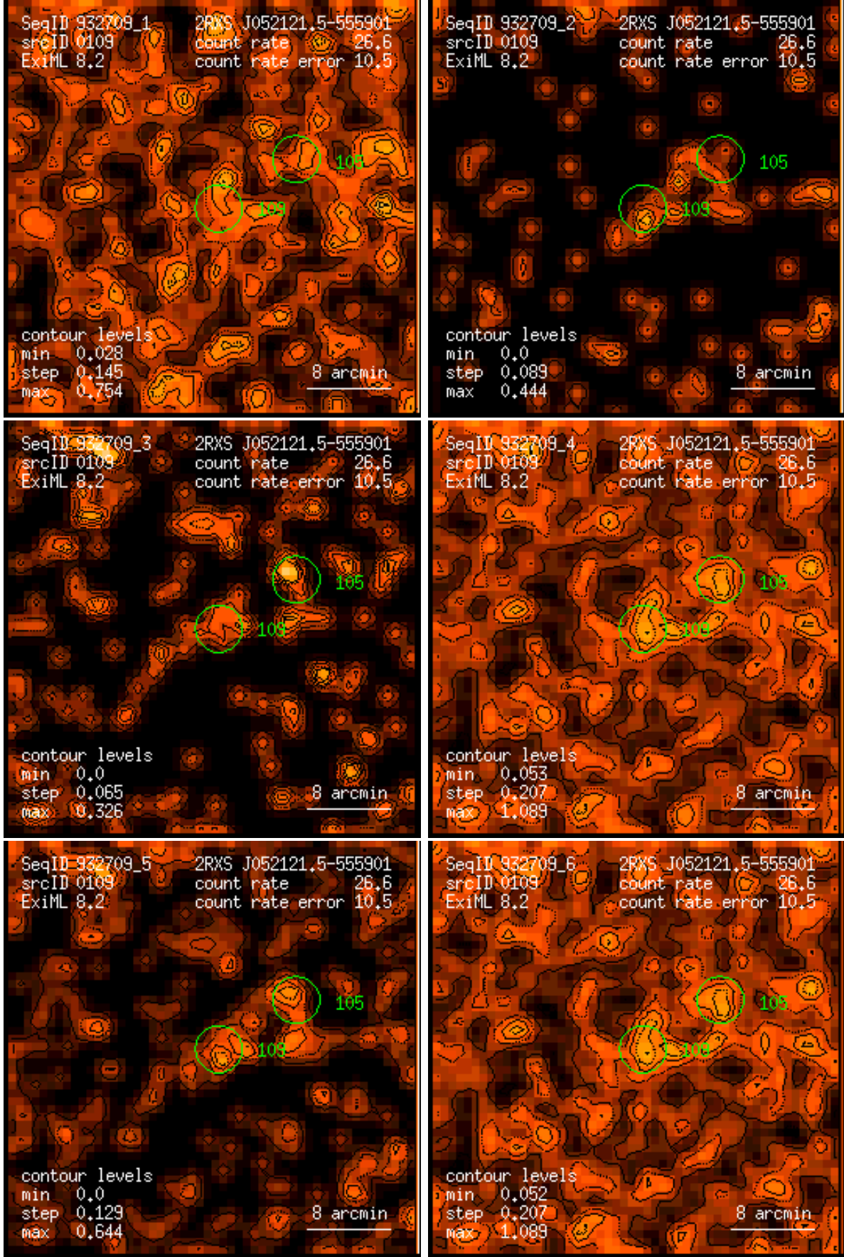
Figure 109: RASS 932709: detection 0109: band rate images, Gaussian filter: (1) PSPC channels 11 – 41, (2) 52 – 90, (3) 91 – 201, (4) 11 – 235, (5) 52 – 201, (6) 11 – 201. Broad band rates in counts/ks. Band rate contour levels in counts/ks/arcmin 2 .
