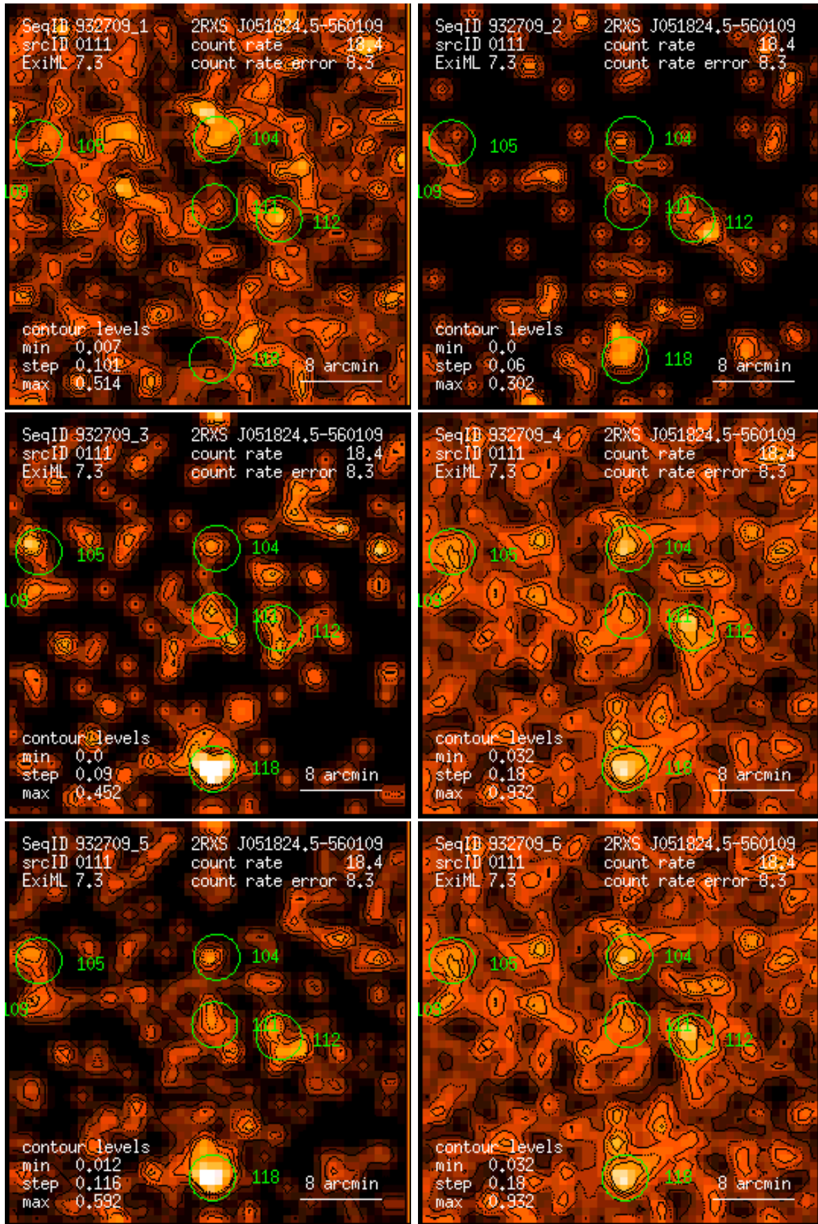
Figure 111: RASS 932709: detection 0111: band rate images, Gaussian filter: (1) PSPC channels 11 – 41, (2) 52 – 90, (3) 91 – 201, (4) 11 – 235, (5) 52 – 201, (6) 11 – 201. Broad band rates in counts/ks. Band rate contour levels in counts/ks/arcmin 2 .
