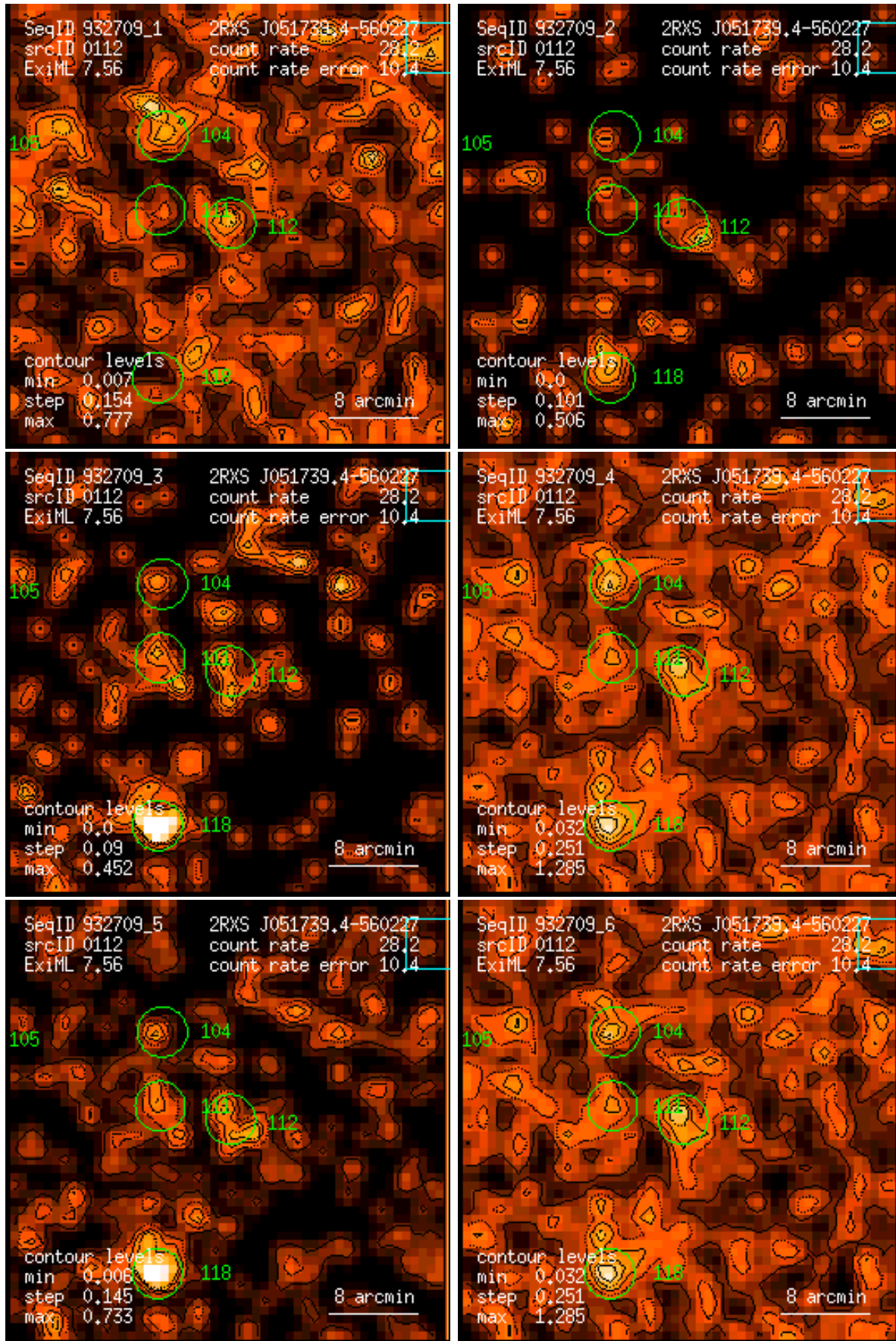
Figure 112: RASS 932709: detection 0112: band rate images, Gaussian filter: (1) PSPC channels 11 – 41, (2) 52 – 90, (3) 91 – 201, (4) 11 – 235, (5) 52 – 201, (6) 11 – 201. Broad band rates in counts/ks. Band rate contour levels in counts/ks/arcmin 2 .
