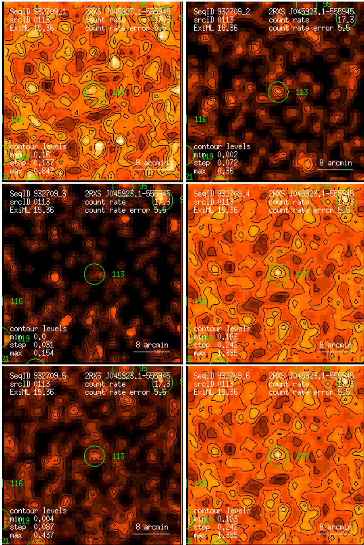
Figure 113: RASS 932709: detection 0113: band rate images, Gaussian filter: (1) PSPC channels 11 – 41, (2) 52 – 90, (3) 91 – 201, (4) 11 – 235, (5) 52 – 201, (6) 11 – 201. Broad band rates in counts/ks. Band rate contour levels in counts/ks/arcmin 2 .
