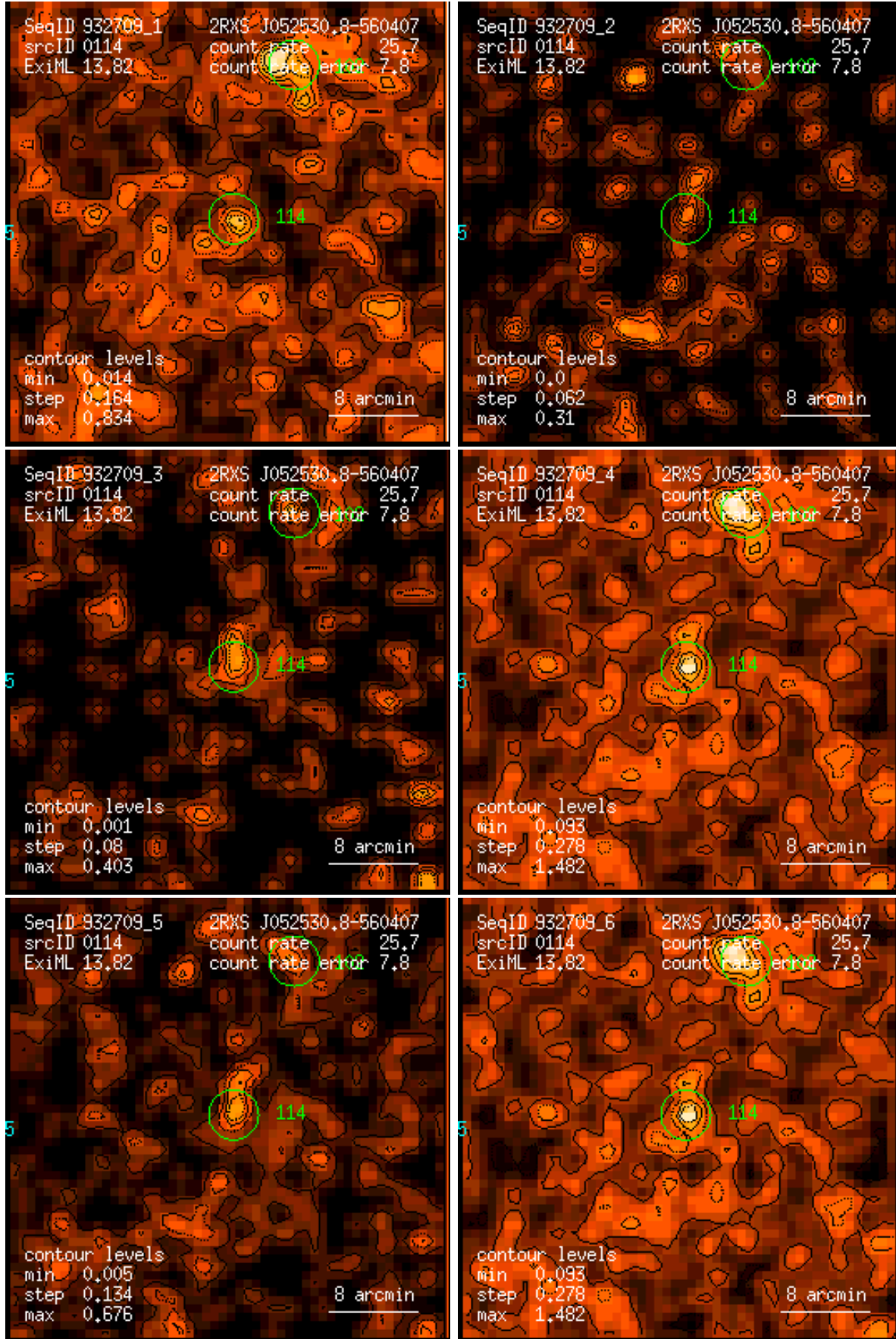
Figure 114: RASS 932709: detection 0114: band rate images, Gaussian filter: (1) PSPC channels 11 – 41, (2) 52 – 90, (3) 91 – 201, (4) 11 – 235, (5) 52 – 201, (6) 11 – 201. Broad band rates in counts/ks. Band rate contour levels in counts/ks/arcmin 2 .
