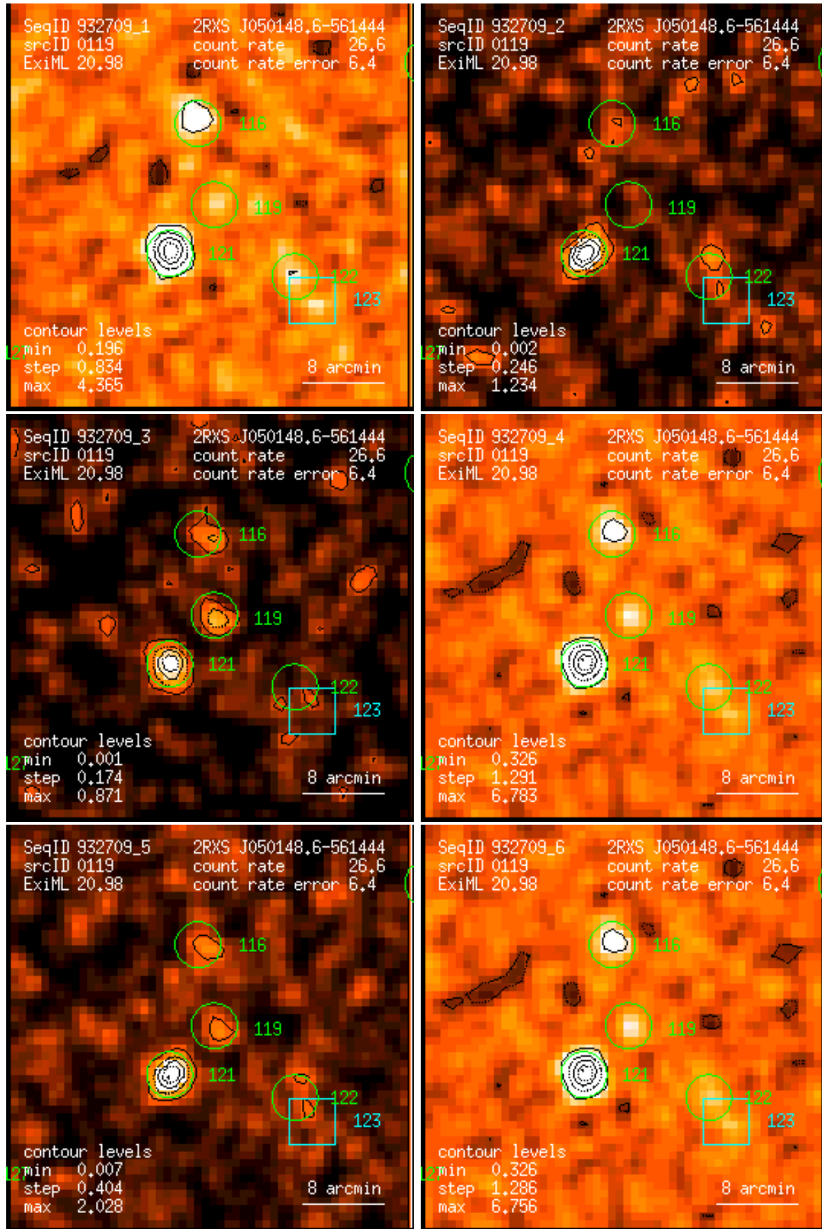
Figure 119: RASS 932709: detection 0119: band rate images, Gaussian filter: (1) PSPC channels 11 – 41, (2) 52 – 90, (3) 91 – 201, (4) 11 – 235, (5) 52 – 201, (6) 11 – 201. Broad band rates in counts/ks. Band rate contour levels in counts/ks/arcmin 2 .
