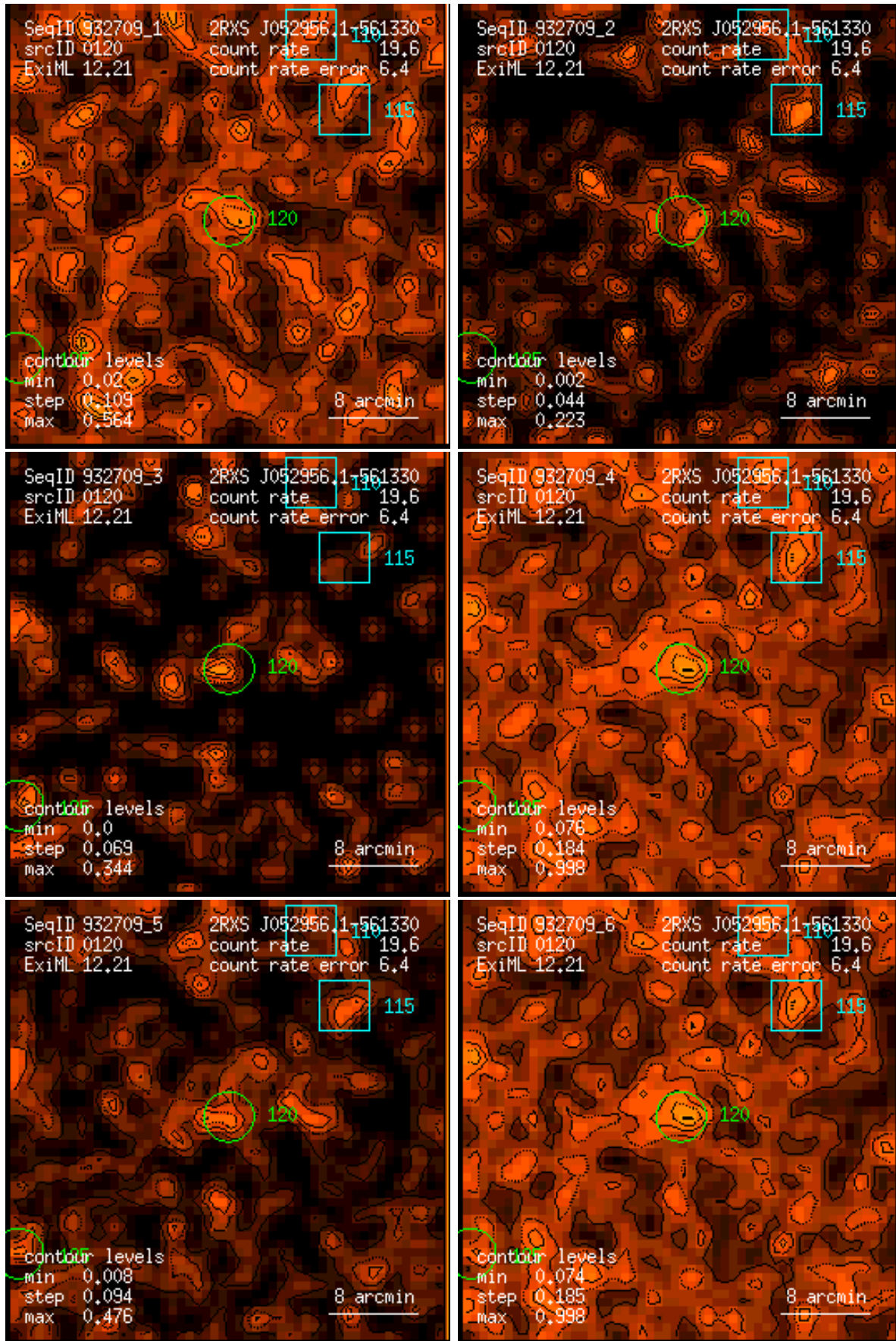
Figure 120: RASS 932709: detection 0120: band rate images, Gaussian filter: (1) PSPC channels 11 – 41, (2) 52 – 90, (3) 91 – 201, (4) 11 – 235, (5) 52 – 201, (6) 11 – 201. Broad band rates in counts/ks. Band rate contour levels in counts/ks/arcmin 2 .
