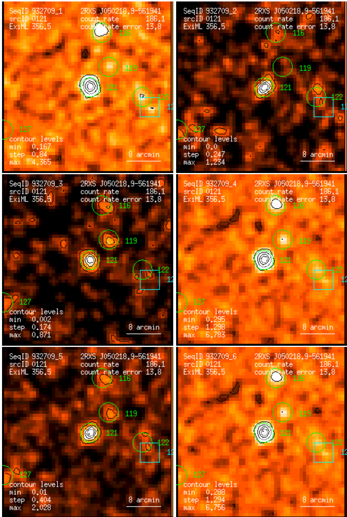
Figure 121: RASS 932709: detection 0121: band rate images, Gaussian filter: (1) PSPC channels 11 – 41, (2) 52 – 90, (3) 91 – 201, (4) 11 – 235, (5) 52 – 201, (6) 11 – 201. Broad band rates in counts/ks. Band rate contour levels in counts/ks/arcmin 2 .
