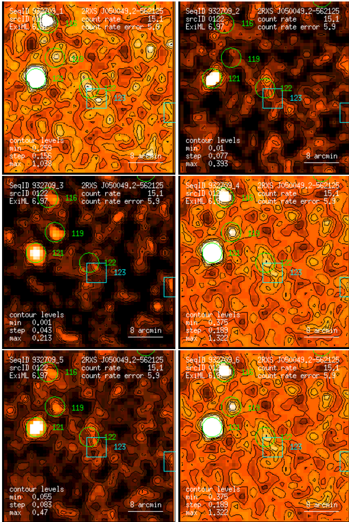
Figure 122: RASS 932709: detection 0122: band rate images, Gaussian filter: (1) PSPC channels 11 – 41, (2) 52 – 90, (3) 91 – 201, (4) 11 – 235, (5) 52 – 201, (6) 11 – 201. Broad band rates in counts/ks. Band rate contour levels in counts/ks/arcmin 2 .
