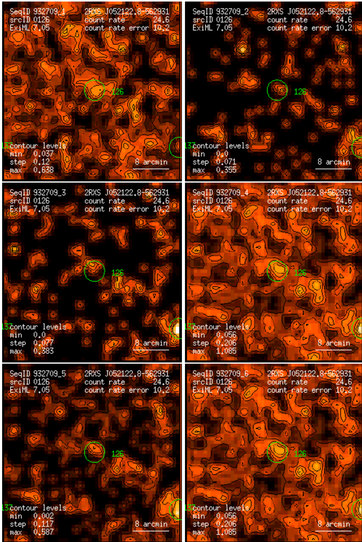
Figure 126: RASS 932709: detection 0126: band rate images, Gaussian filter: (1) PSPC channels 11 – 41, (2) 52 – 90, (3) 91 – 201, (4) 11 – 235, (5) 52 – 201, (6) 11 – 201. Broad band rates in counts/ks. Band rate contour levels in counts/ks/arcmin 2 .
