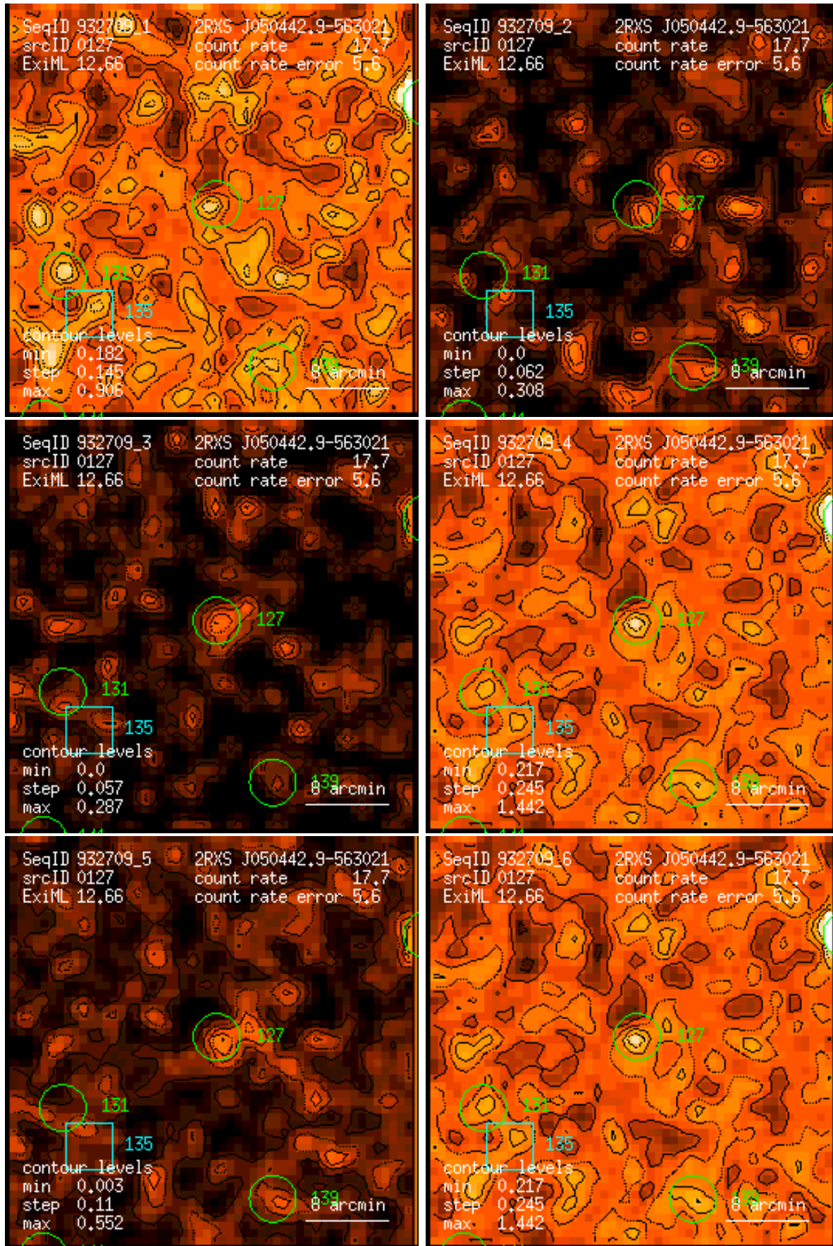
Figure 127: RASS 932709: detection 0127: band rate images, Gaussian filter: (1) PSPC channels 11 – 41, (2) 52 – 90, (3) 91 – 201, (4) 11 – 235, (5) 52 – 201, (6) 11 – 201. Broad band rates in counts/ks. Band rate contour levels in counts/ks/arcmin 2 .
