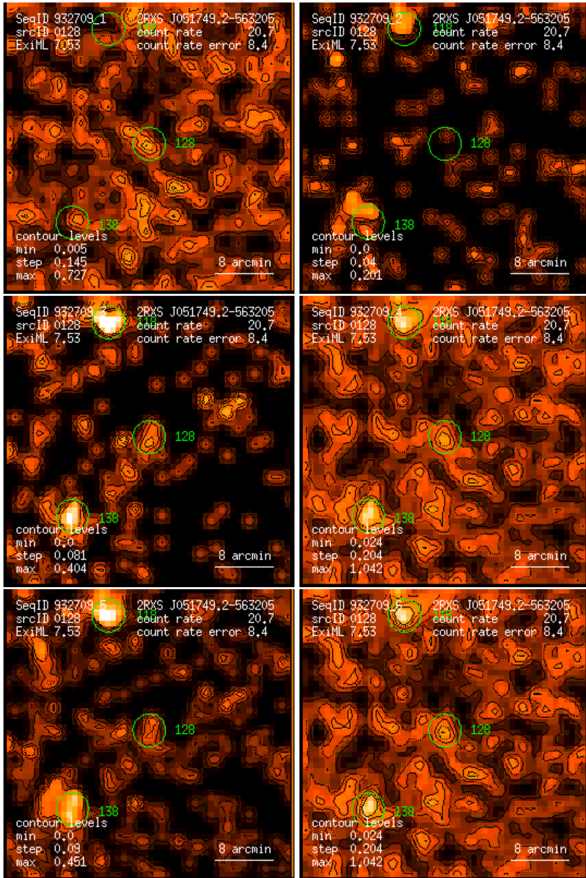
Figure 128: RASS 932709: detection 0128: band rate images, Gaussian filter: (1) PSPC channels 11 – 41, (2) 52 – 90, (3) 91 – 201, (4) 11 – 235, (5) 52 – 201, (6) 11 – 201. Broad band rates in counts/ks. Band rate contour levels in counts/ks/arcmin 2 .
